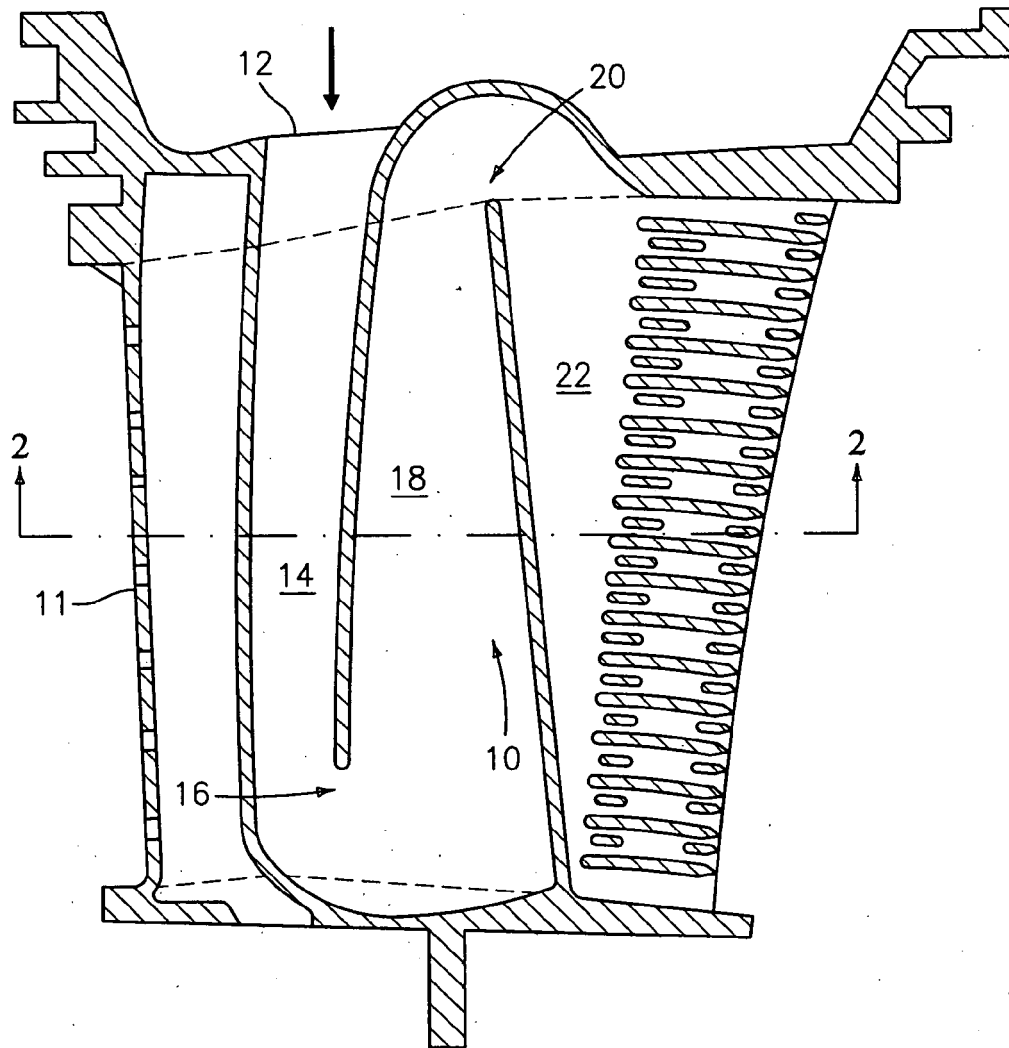
FIG. 1 (PRIOR ART)
