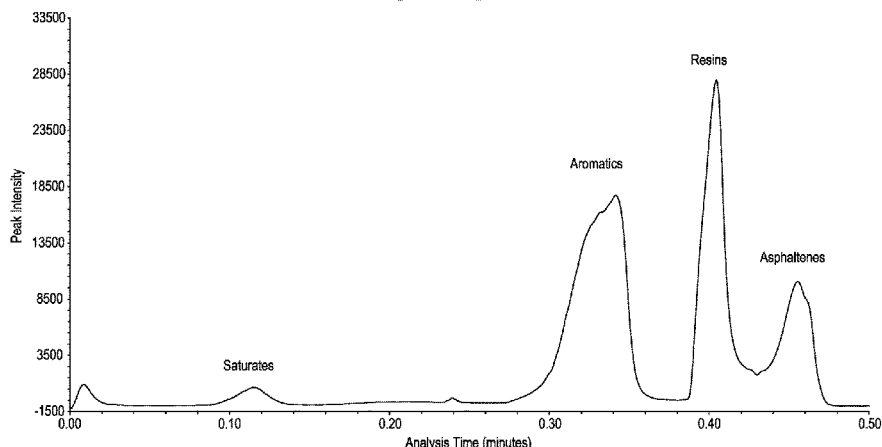
Iatroscan Chromatogram, Virgin 70/100 Bitumen
