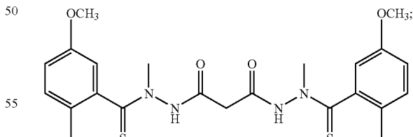
Compound (14)
