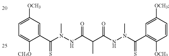
Compound (10)
