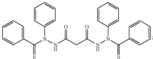
Compound (4)
