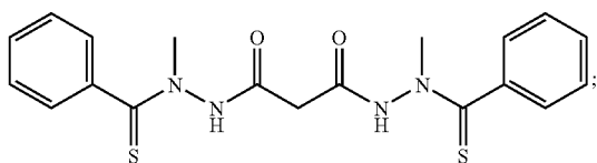
Compound (2)
