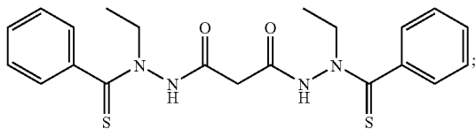
Compound (5)
