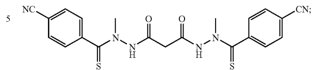
Compound (8)
