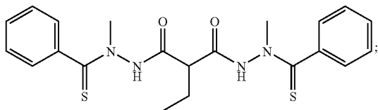
Compound (6)
