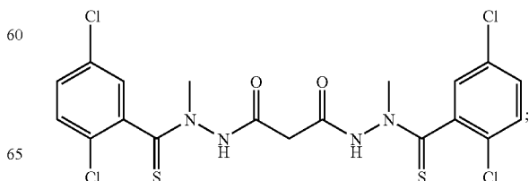
Compound (14)
