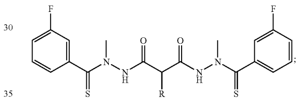
Compound (11)
