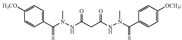
Compound (6)
