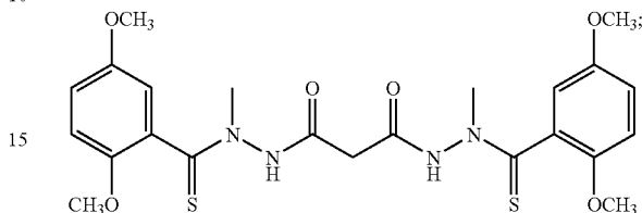
Compound (9)
