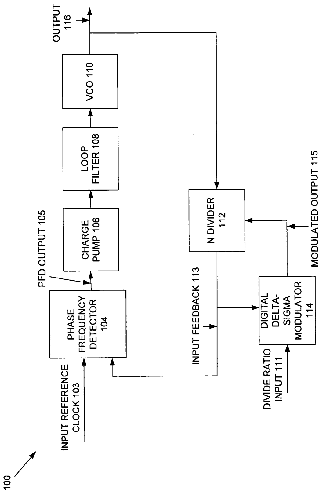
FIGURE 1 - PRIOR ART
