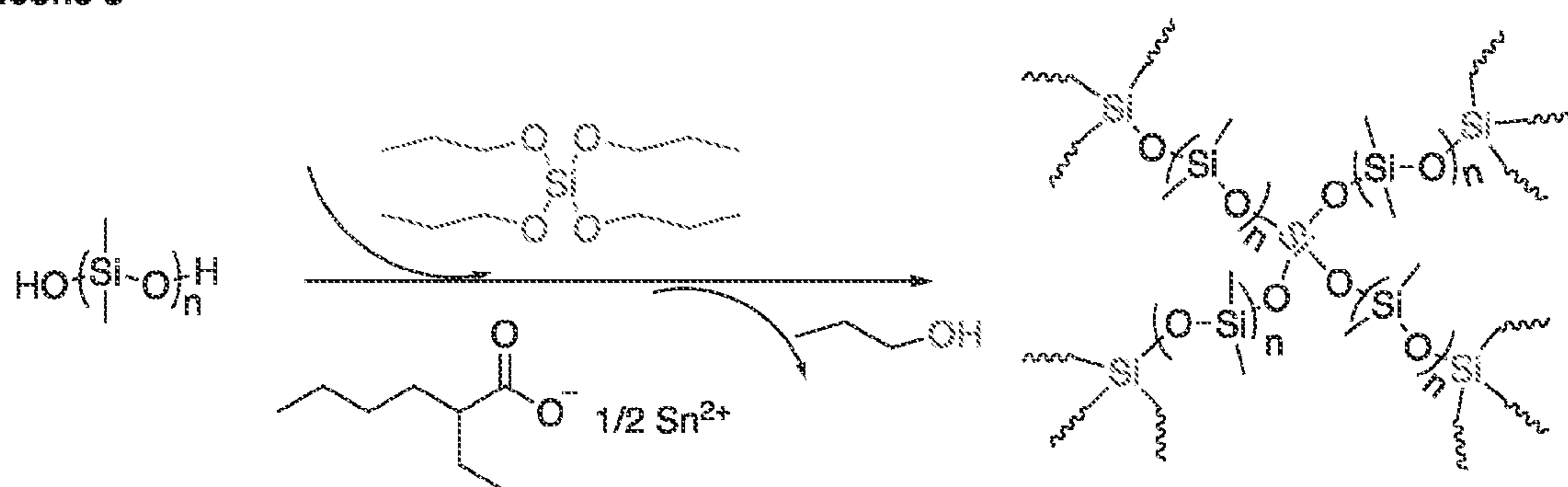
Scheme 1. Curing chemistries of representative fluorosilicones and silicones studied in this work (see also Table 1).
