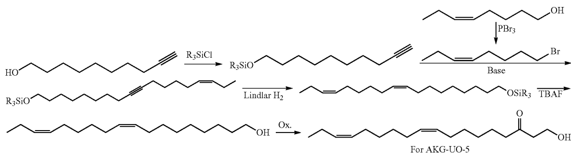
Scheme 2 Synthesis of acid intermediate for AKG-UO-5
