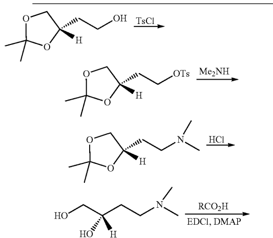
Scheme 4 Synthesis of AKG-UO-1, AKG-UO-4, AKG-UO-5, AKG-BDG-1 and AKG-BDG-2
