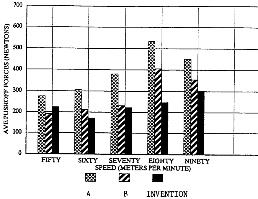
Wet turning tests on paarl granite showing (change in speed VS pushoff forces)
