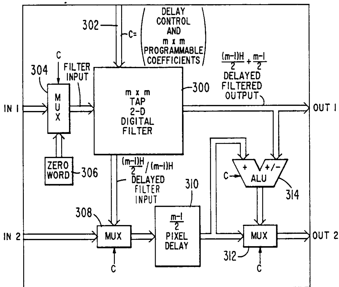
FILTER LOGIC UNIT MODULE
