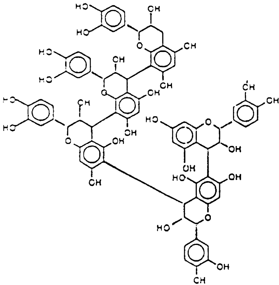
(4-E) (4-B) (4-B) (4-B) pentamer
