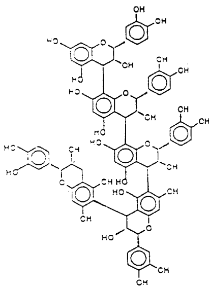
(4-E) (4-E) (4-E) (4-E) pentamer
