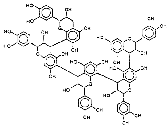
(4-E) (4-E) (4-E) (4-E) pentamer
