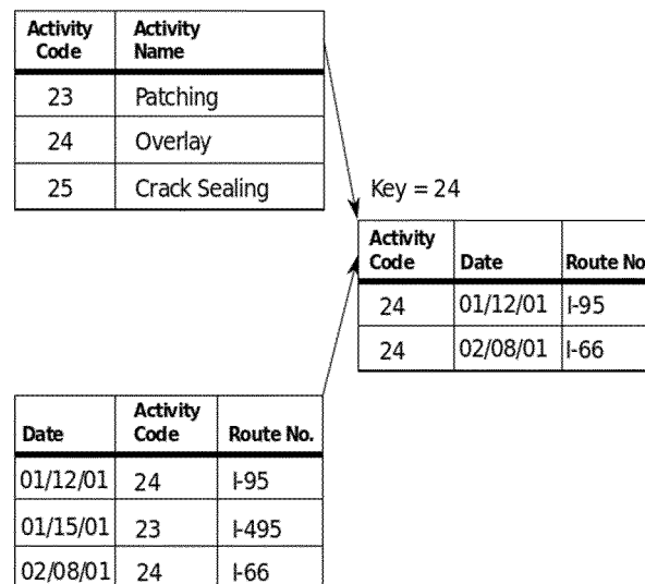
Relational Model
