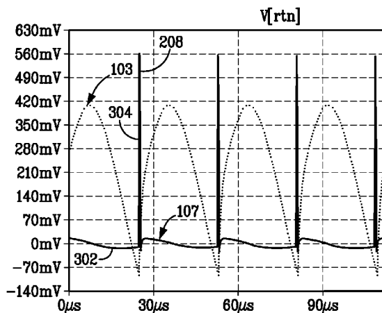
At Resonance
