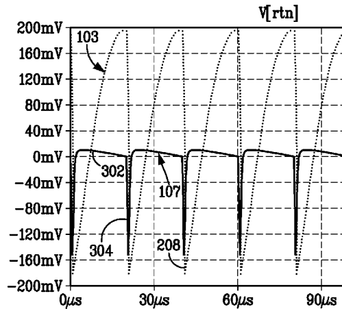
Above Resonance
