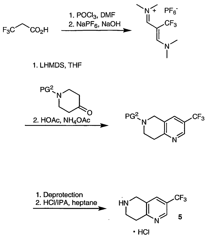
Scheme 4A
