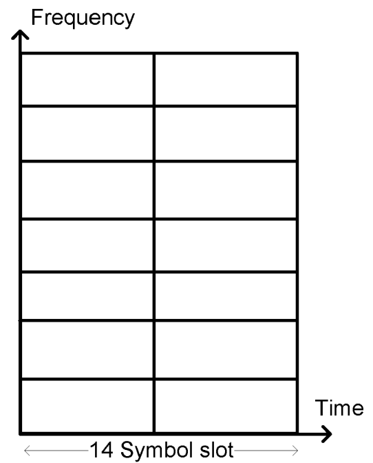
(B) 1 bit in bitmap indicates 1/7^{\text{th}} of PRBs over one half-slot (7 symbols).
