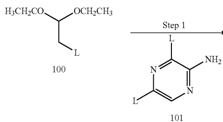
Reaction Scheme 1
