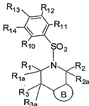
Formula 6
