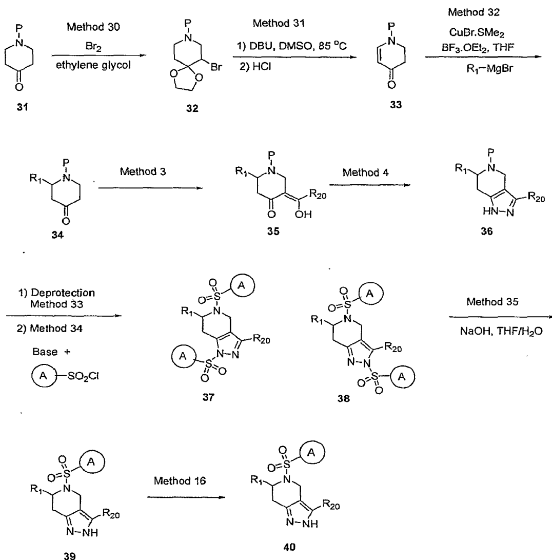
Scheme 4:
