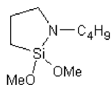
Structure 1. Cyclic Azasilane N-n-BUTYL-AZA-2,2-DIMETHOXY SILACYCLOPENTANE
