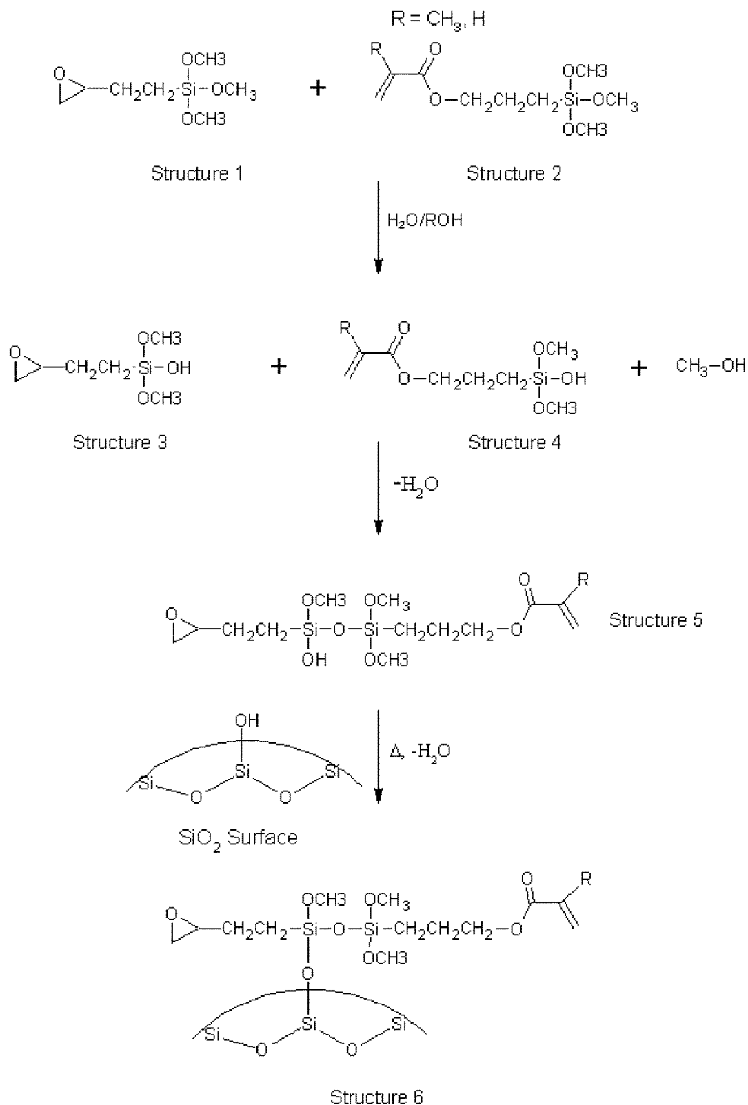
FIG. 1 (Related Art)
