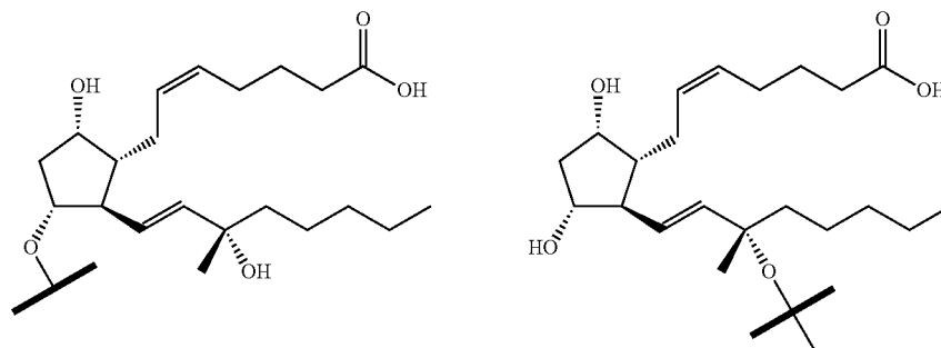
Carboprost
