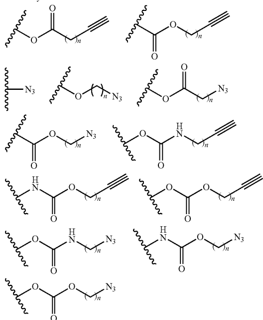
Co-monomers
