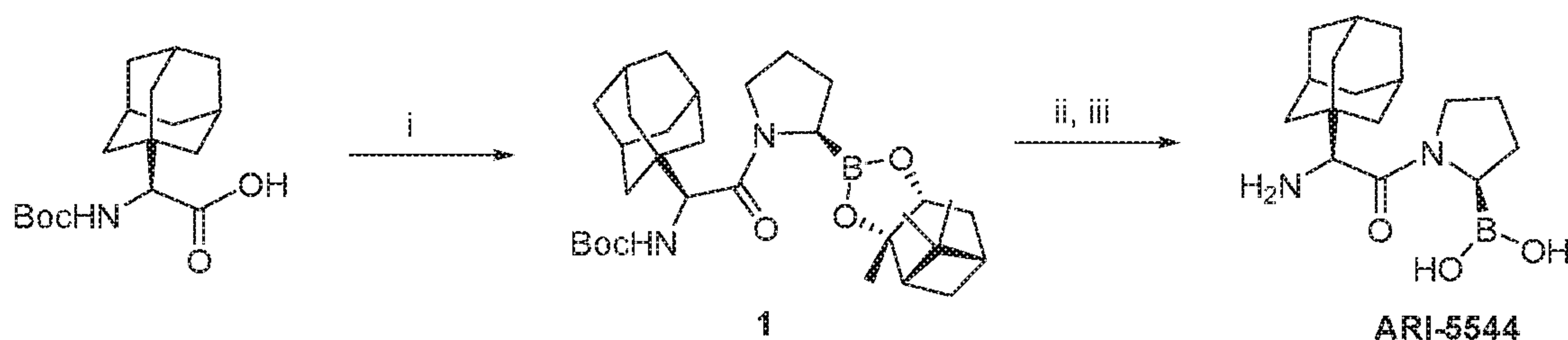
Scheme 2. Synthetic method for ARI-5544 a
