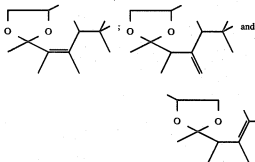
FIG. 15 sets forth the GLC profile for the reaction product produced according to Example IX(A) containing the compounds defined according to the generic structure:
