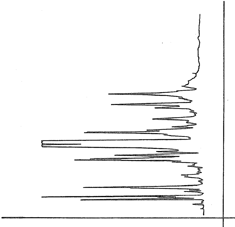
GLC PROFILE FOR EXAMPLE A. FIG.AC
