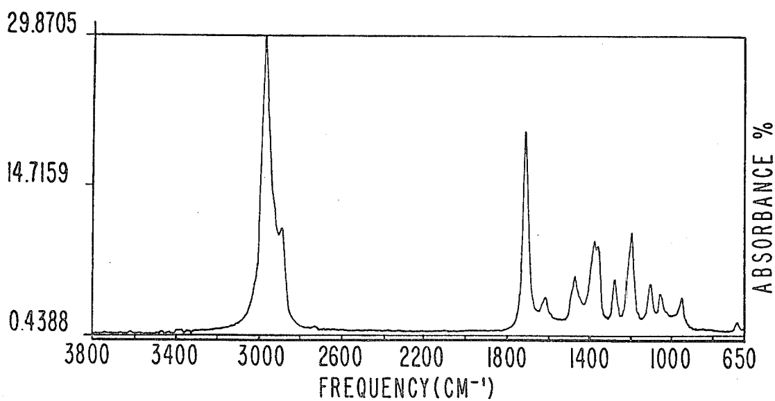
IR SPECTRUM FOR PEAK 7 OF EXAMPLE I.
