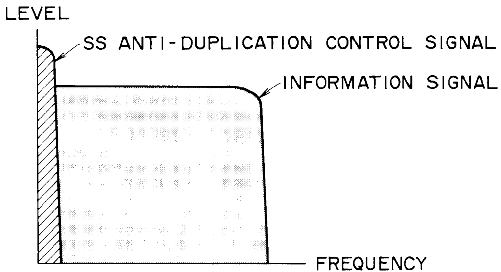
SIGNAL SPECTRUM AFTER SPECTRAL DESPREADING ON RECORDER SIDE
