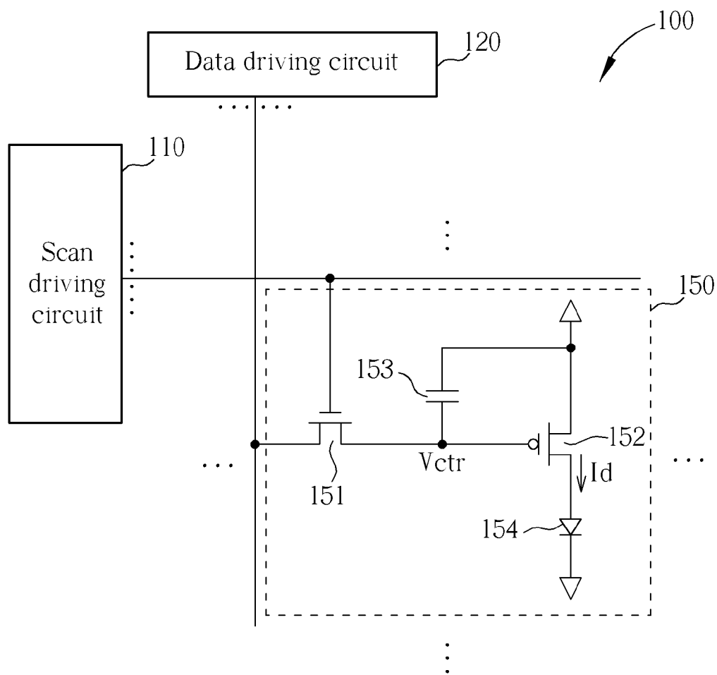
FIG. 1 PRIOR ART
