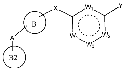
Formula Ia
