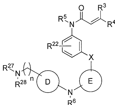
Formula Id
