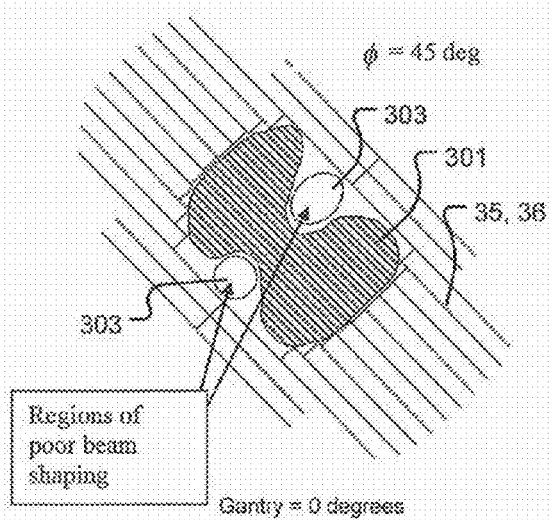
Gantry = 0 degrees FIGURE 18C
