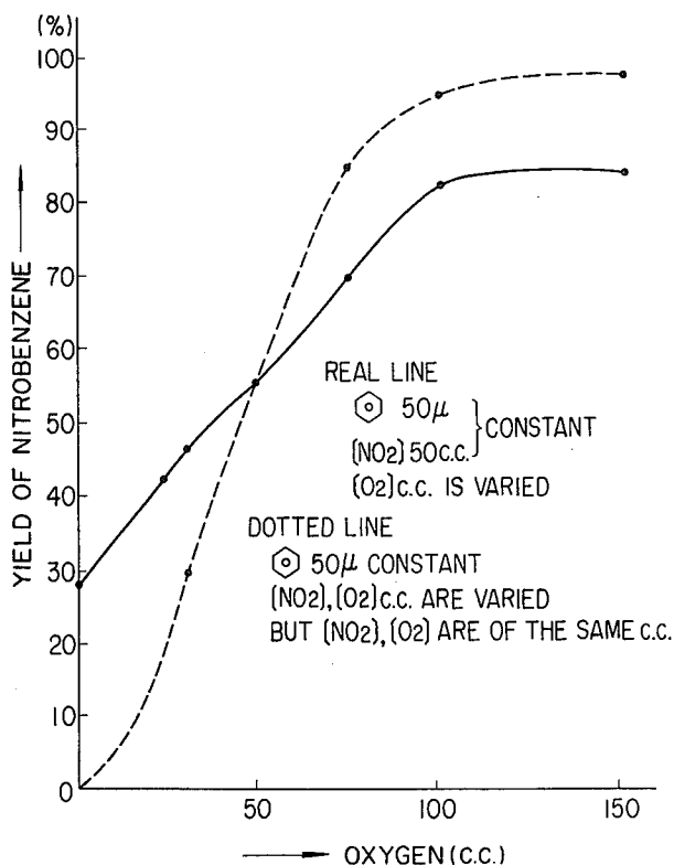
INFLUENCE OF OXYGEN IN NITRATION
