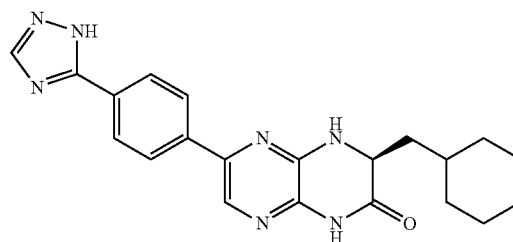
(R)-6-(4-(1H-1,2,4-triazol-5-yl)phenyl)-3-(cyclohexylmethyl)-3,4-dihydropyrazino[2,3-b]pyrazin-2(1H)-one
