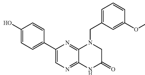
6-(4-hydroxyphenyl)-4-(3-methoxybenzyl)-3,4-dihydropyrazino[2,3-b]pyrazin-2(1H)-one
