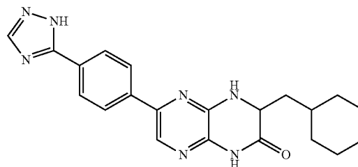
6-(4-(1H-1,2,4-triazol-5-yl)phenyl)-3-(cyclohexylmethyl)-3,4-dihydropyrazino[2,3-b]pyrazin-2(1H)-one
