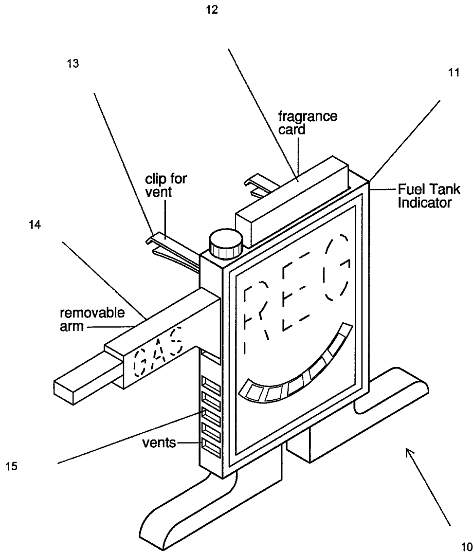
FIG. 1 (ISO View)
