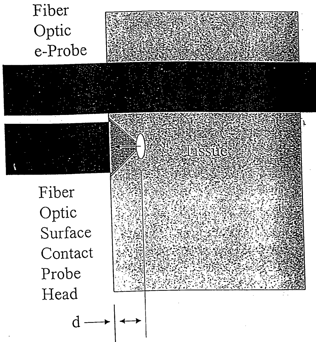
E-probe for pierced ears
