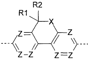
FORMEL (I)
