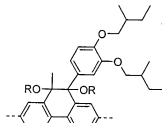
Formel (LXXXXV)
