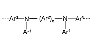
Formel (II)
