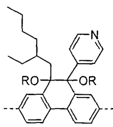
Formel (CIII)
