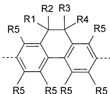
FORMEL (Ib)
