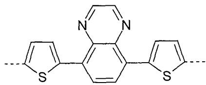
Formel (XXXXI)
