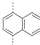
Formel (LXII)
