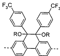
Formel (LXXXIX)
