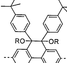
Formel (LXXXVI)
