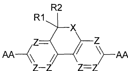
FORMEL (CV)
