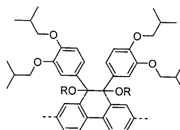
Formel (LXXXVIII)
