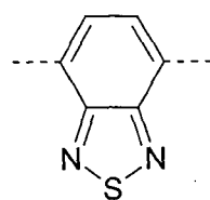
Formel (XXX)
