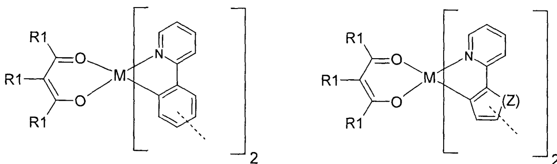
Formel (LVI)
