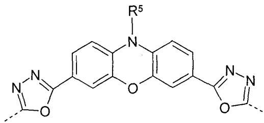
Formel (XXXXIII)
