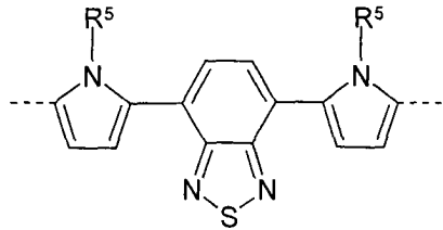
Formel (XXXVI)
