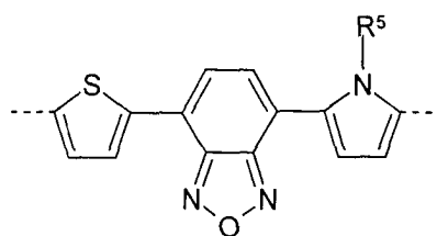
Formel (XXXIX)
