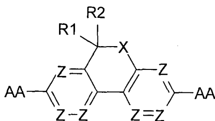
FORMEL (CV)
