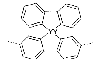
Formel (LXXV)
