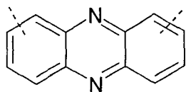
Formel (XXVIII)
