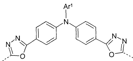
Formel (XXXXII)
