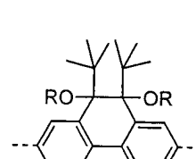
Formel (LXXXII)
