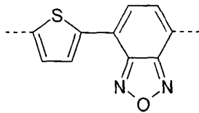
Formel (XXXIV)
