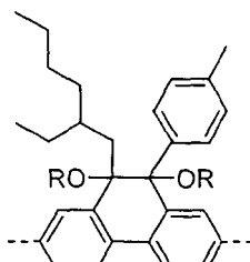
Formel (C)
