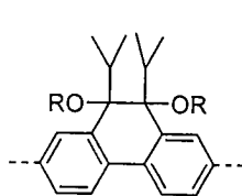
Formel (LXXX)
