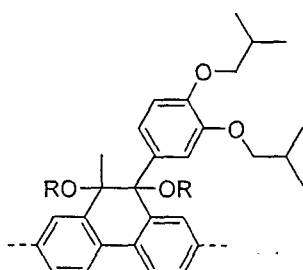
Formel (LXXXVII)
