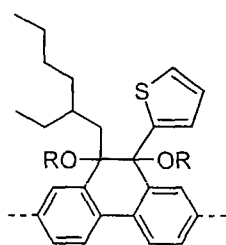
Formel (CII)
