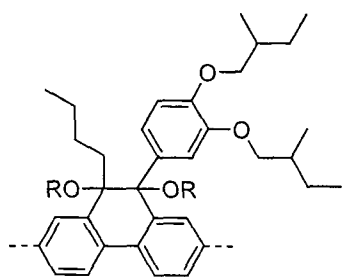
Formel (LXXXVI)
