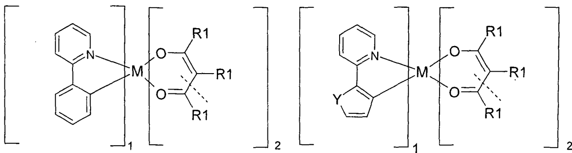
Formel (LIII)
