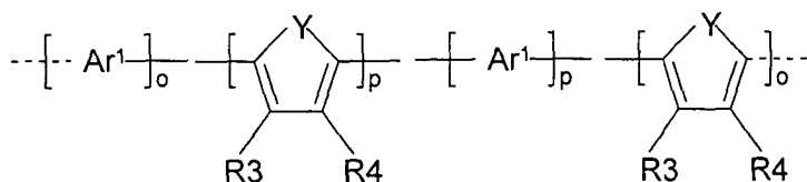
Formel (XXXXVIII)
