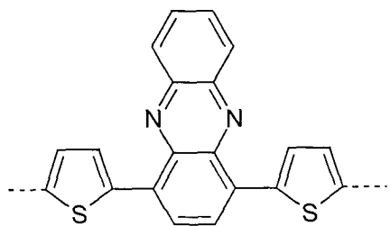
Formel (XXXX)
