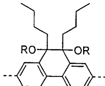
Formel (LXXXI)
