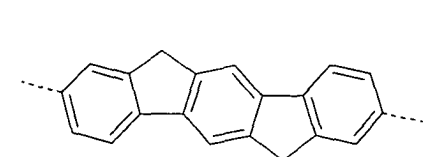
Formel (LXXVII)
