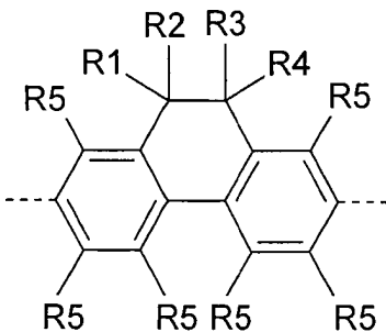
FORMEL (Ib)
