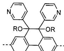
Formel (LXXXXI)
