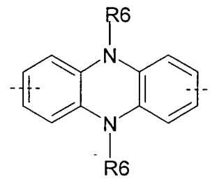
Formel (IX)
