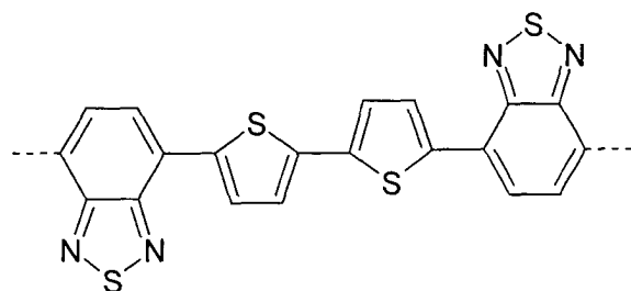
Formel (XXXXVI)
