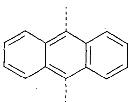
Formel (LXIII)
