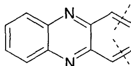
Formel (XXIX)
