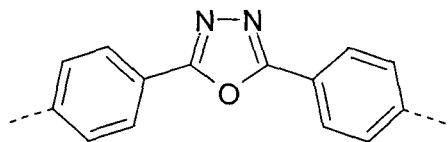
Formel (XXV)
