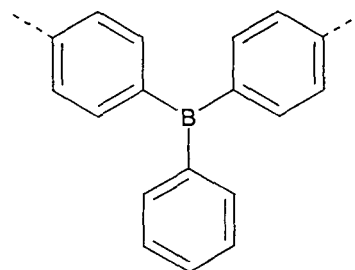
Formel (XXXII)
