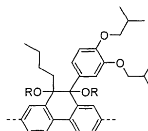
Formel (LXXXVIII)
