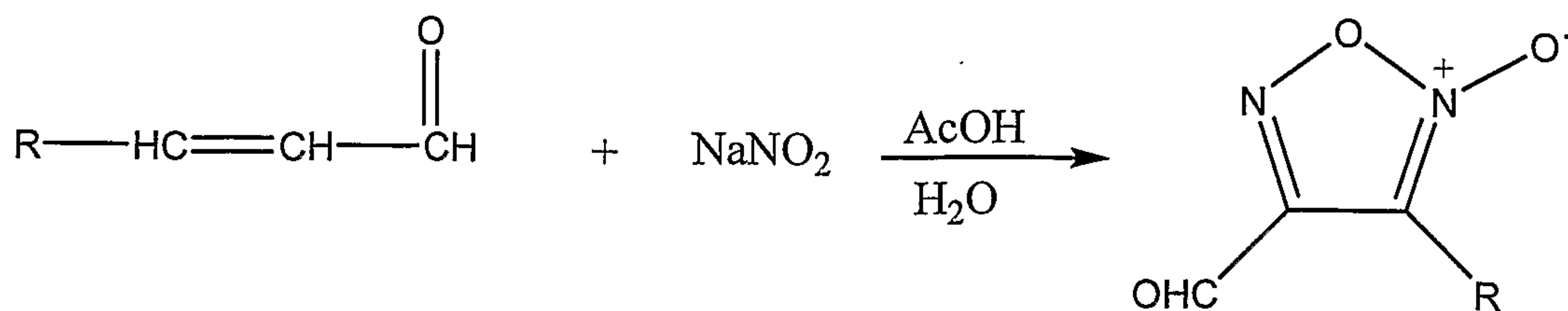
Scheme 3
