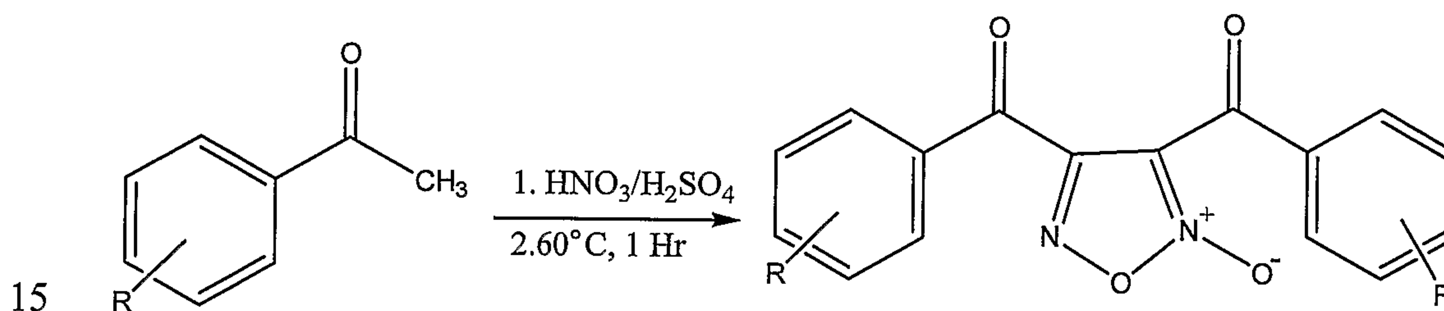
Scheme 4
