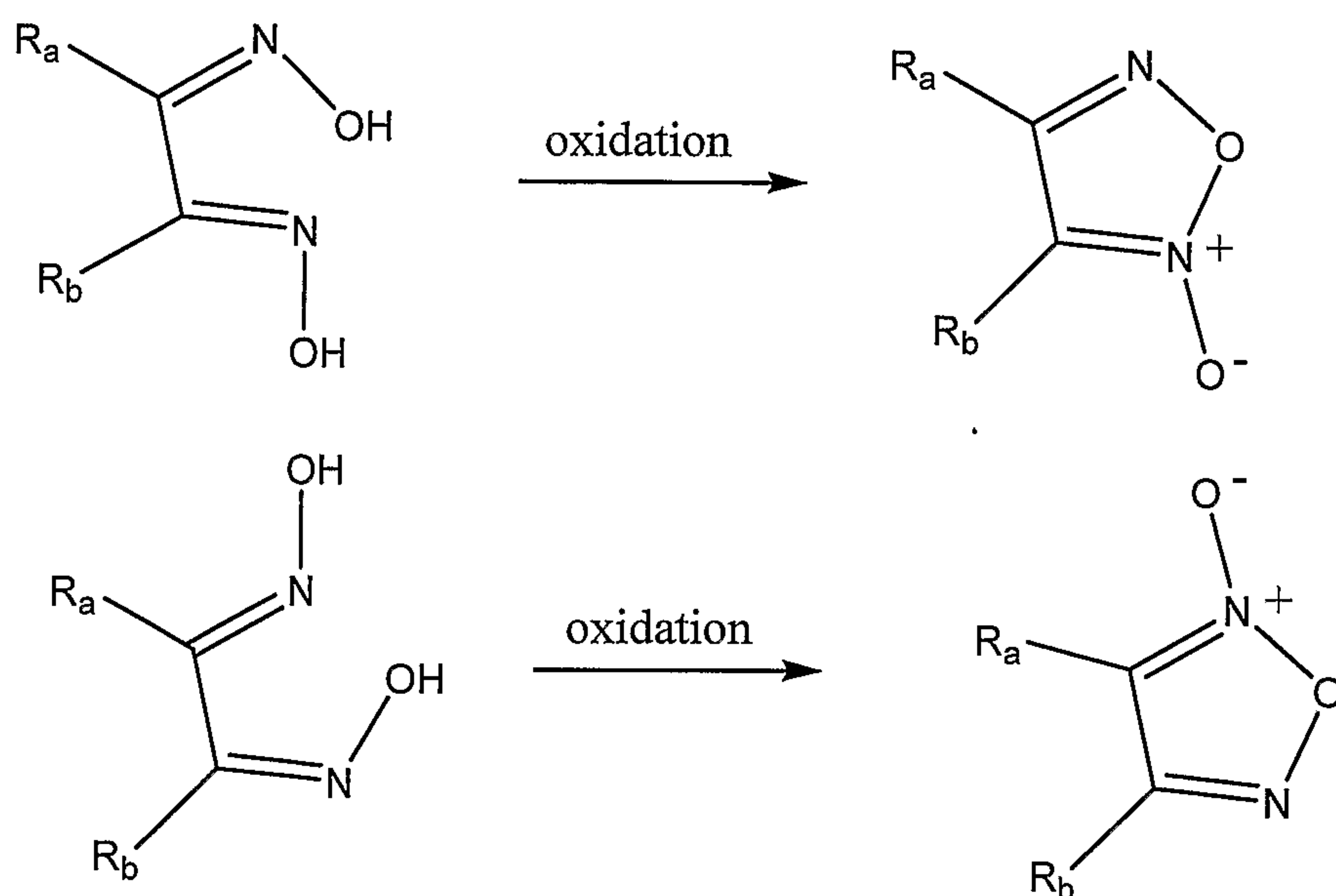
Scheme 2
