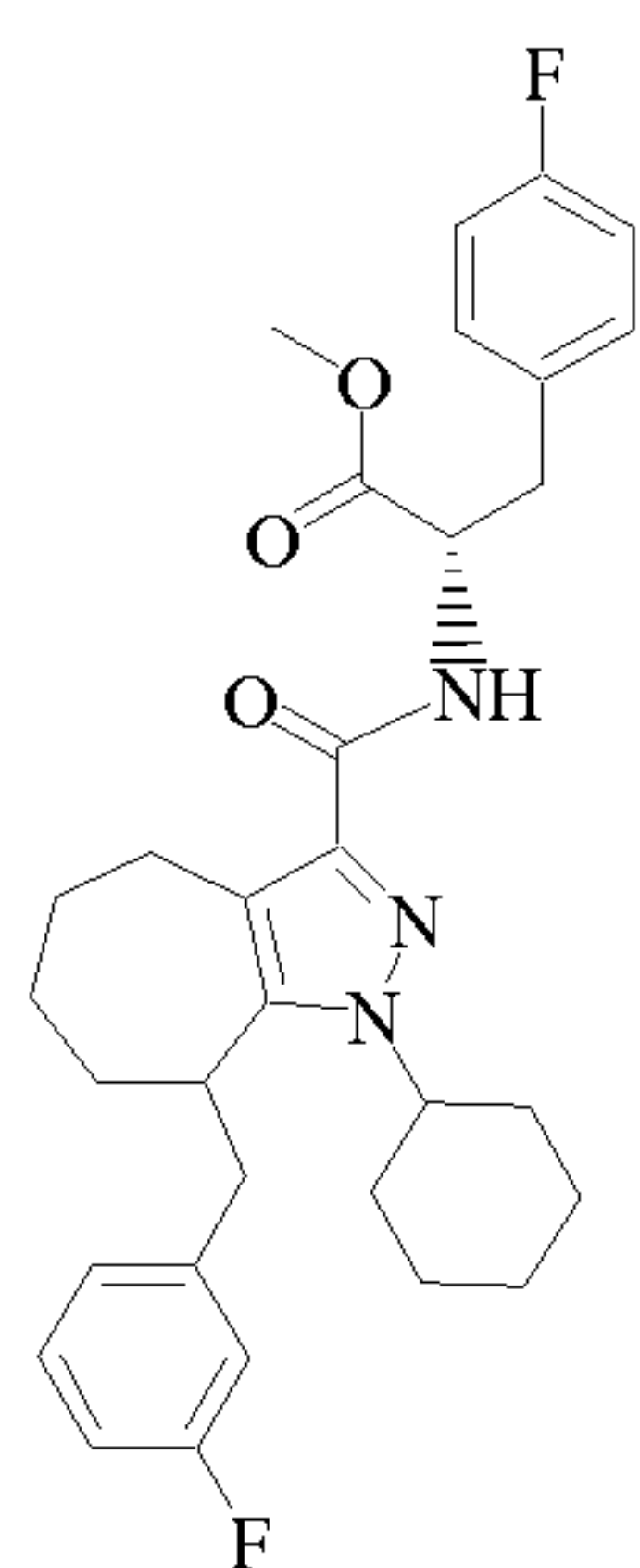
Cpd 73
