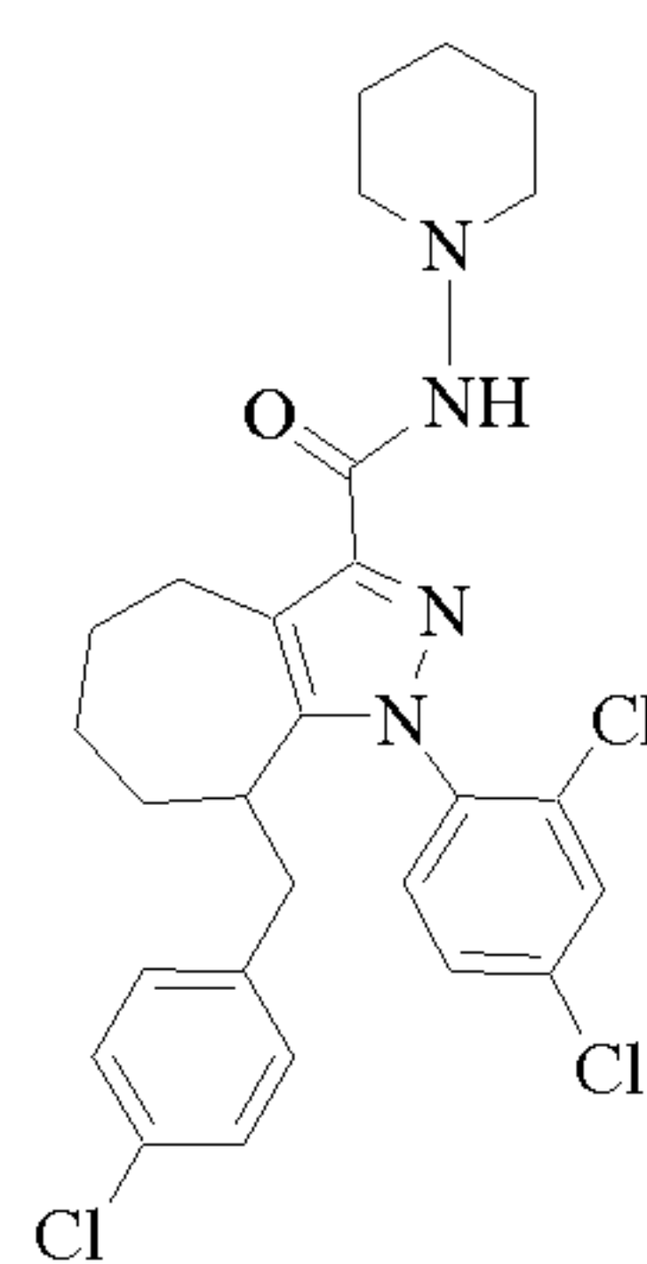
Cpd 27
