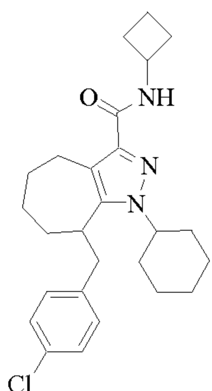
Cpd 37
