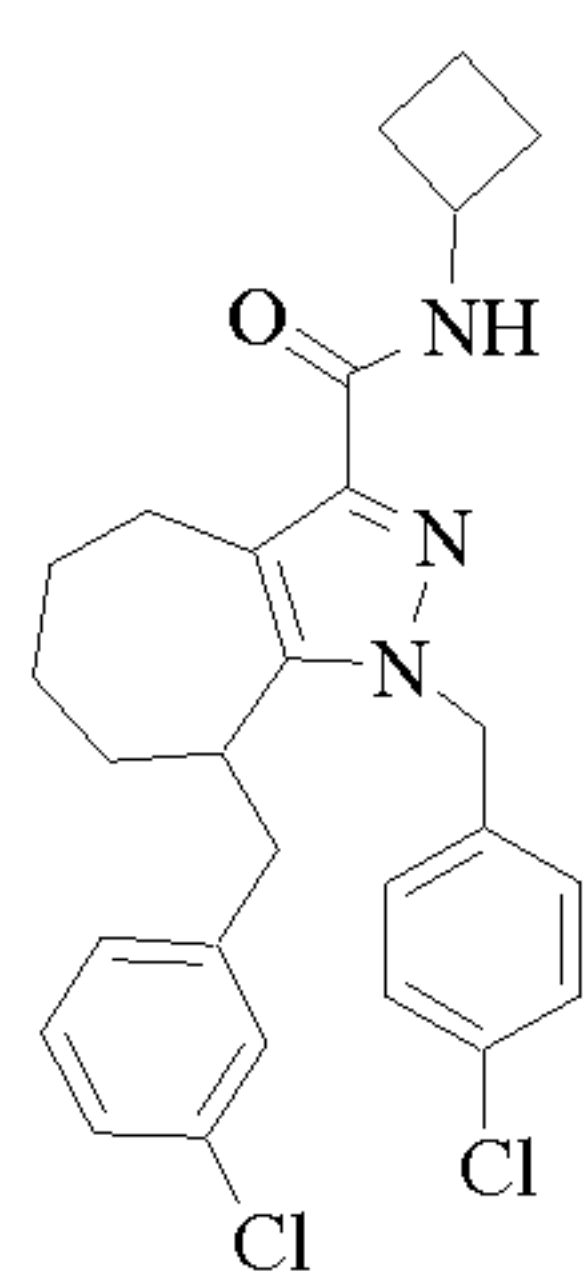
Cpd 29
