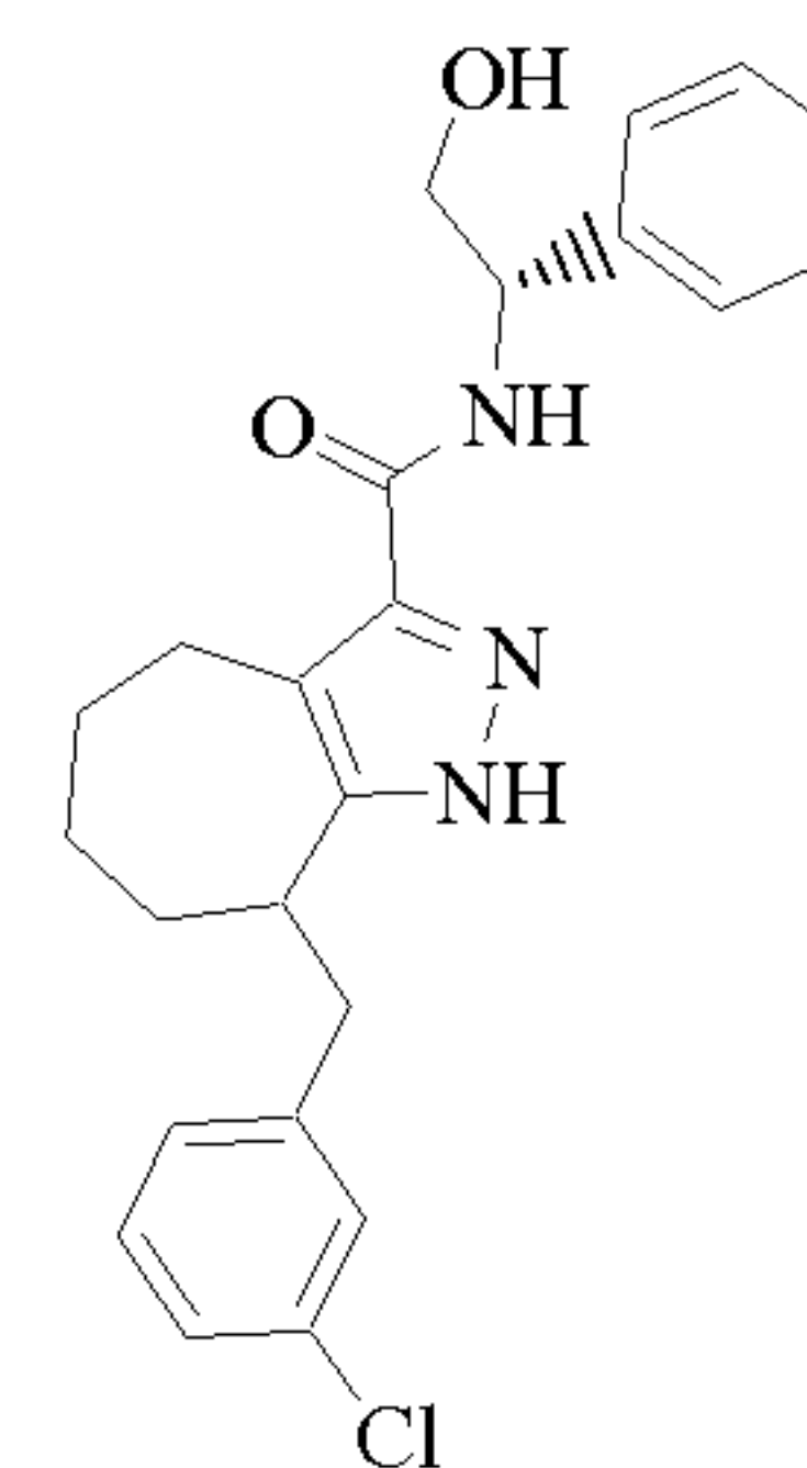
Cpd 164
