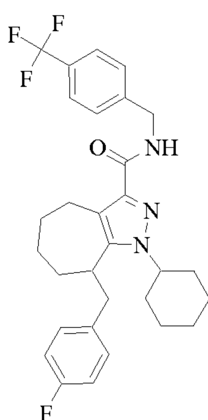
Cpd 65
