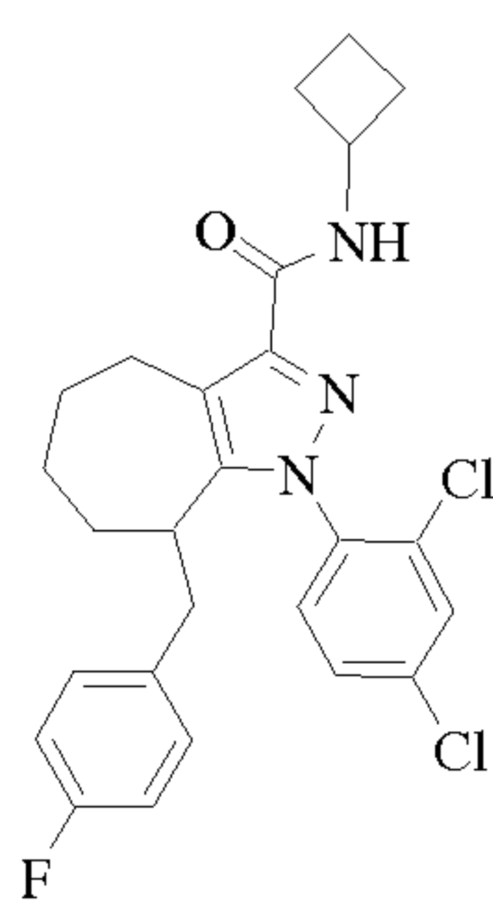
Cpd 66
