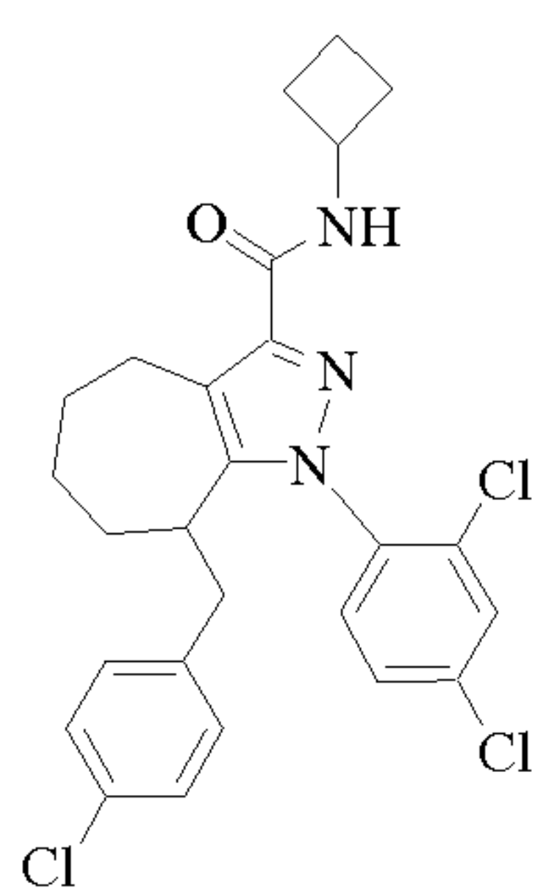
Cpd 21
