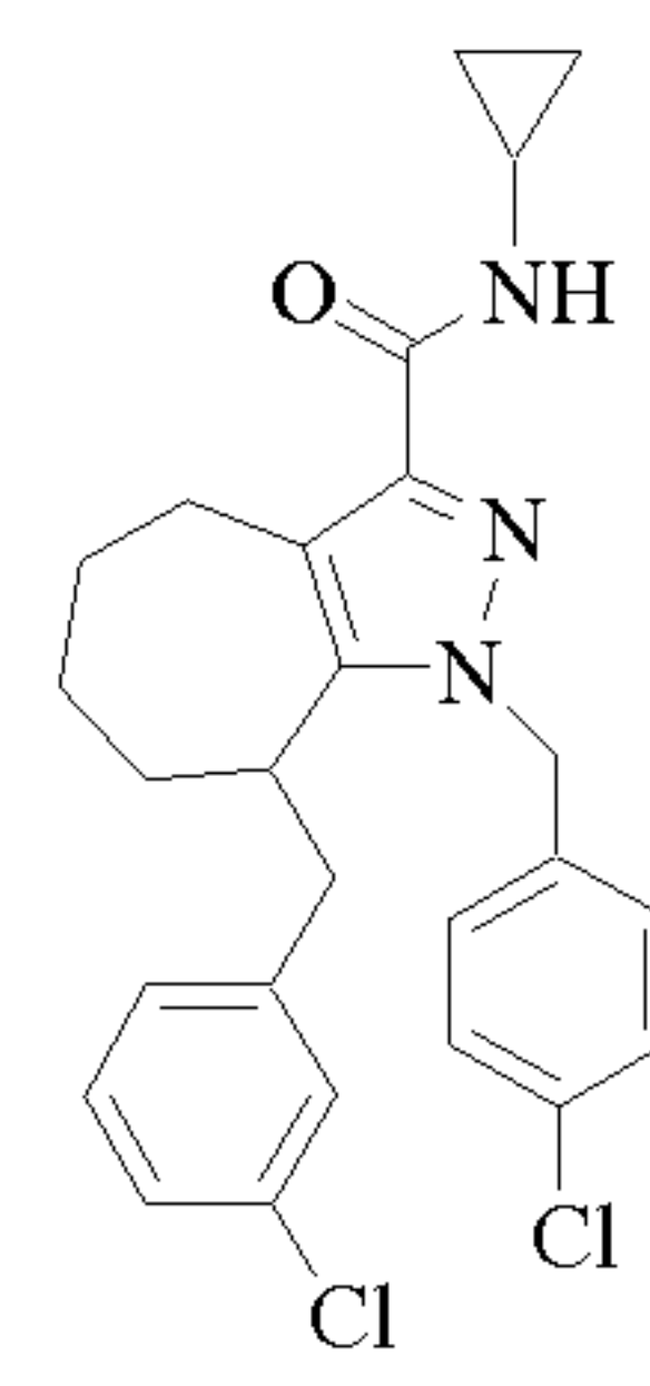
Cpd 35
