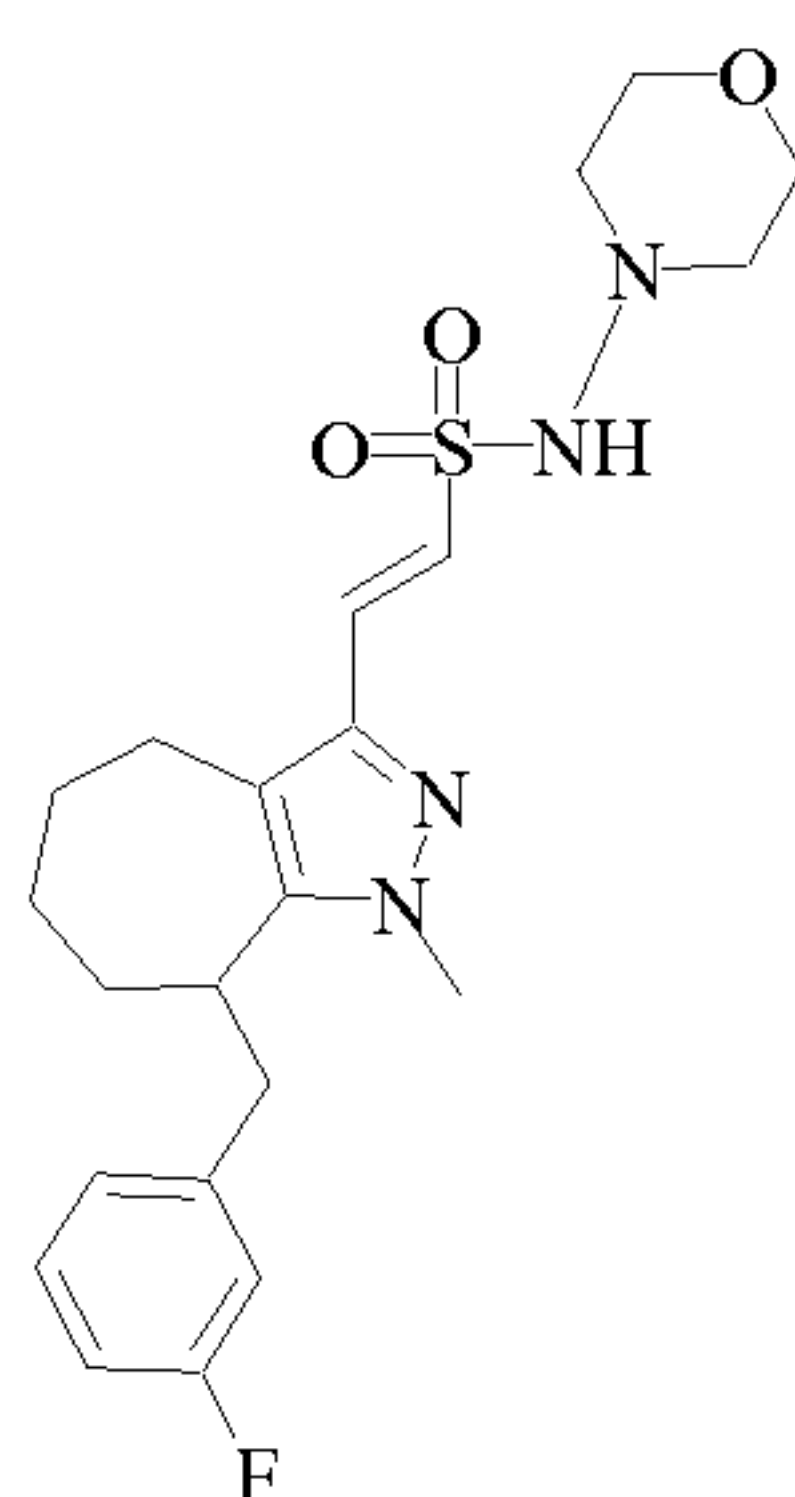
Cpd 125
