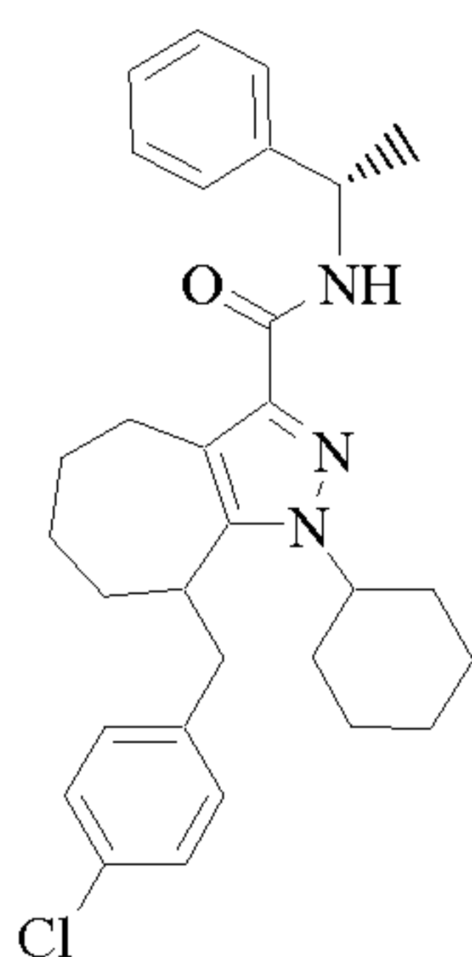
Cpd 1
