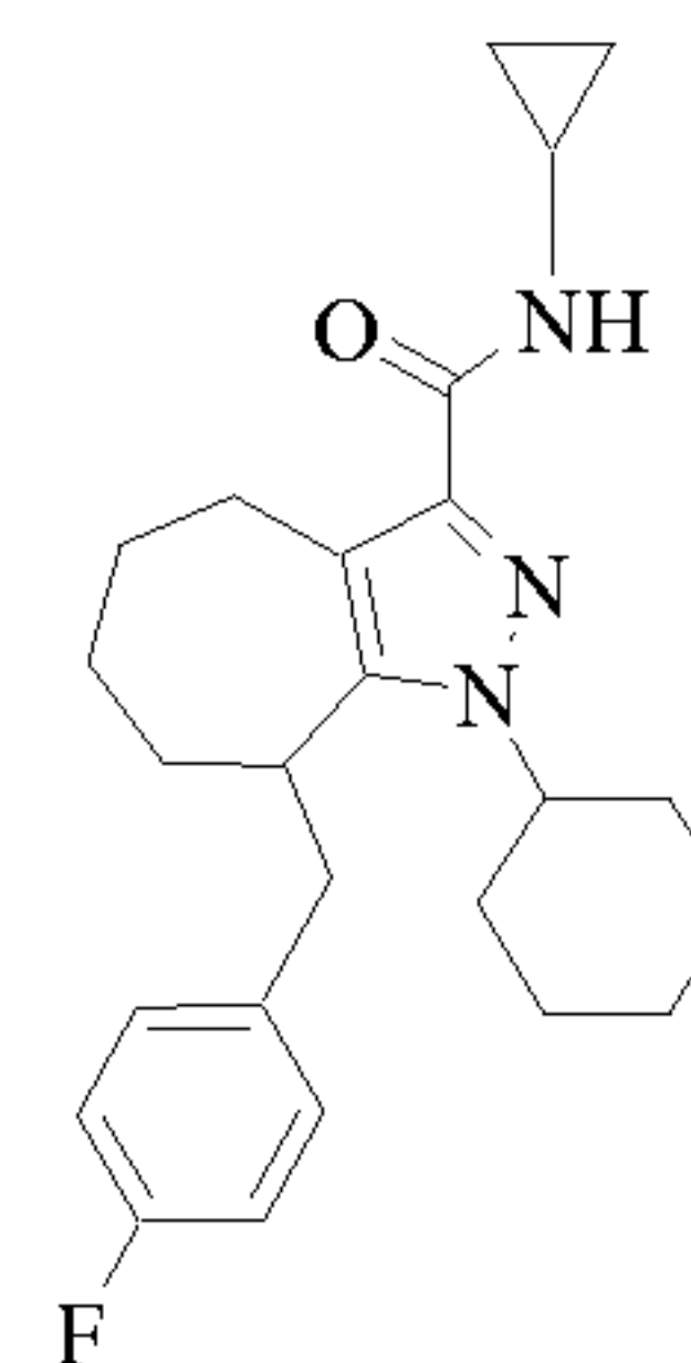
Cpd 52
