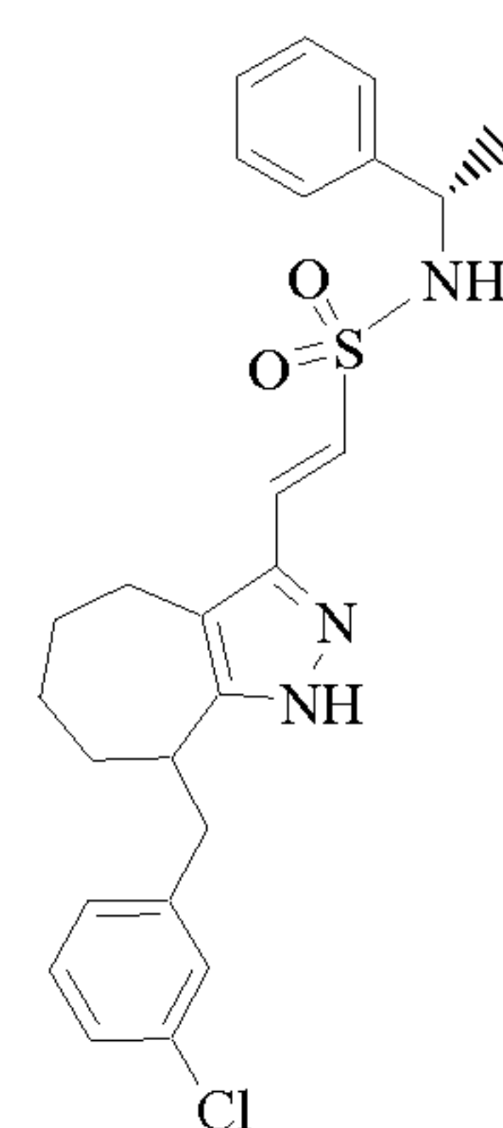
Cpd 160
