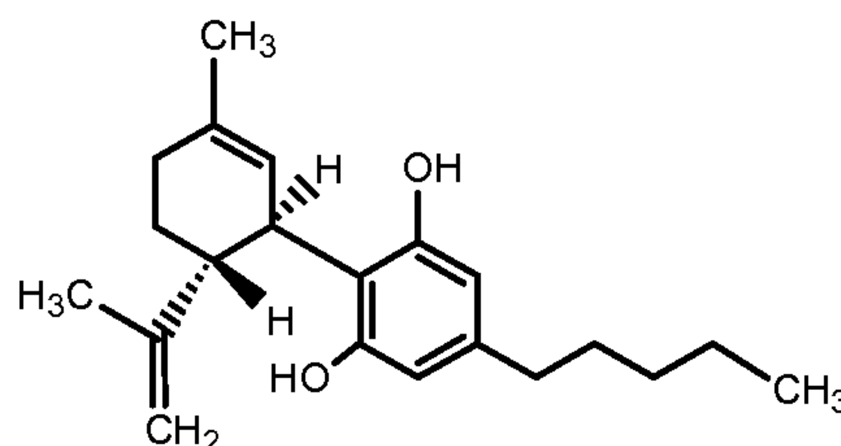
CANNABIDIOL
