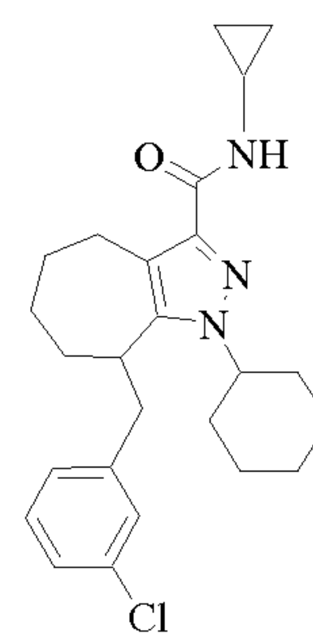
Cpd 32
