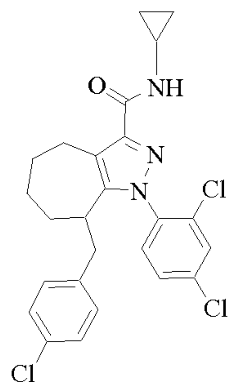
Cpd 38
