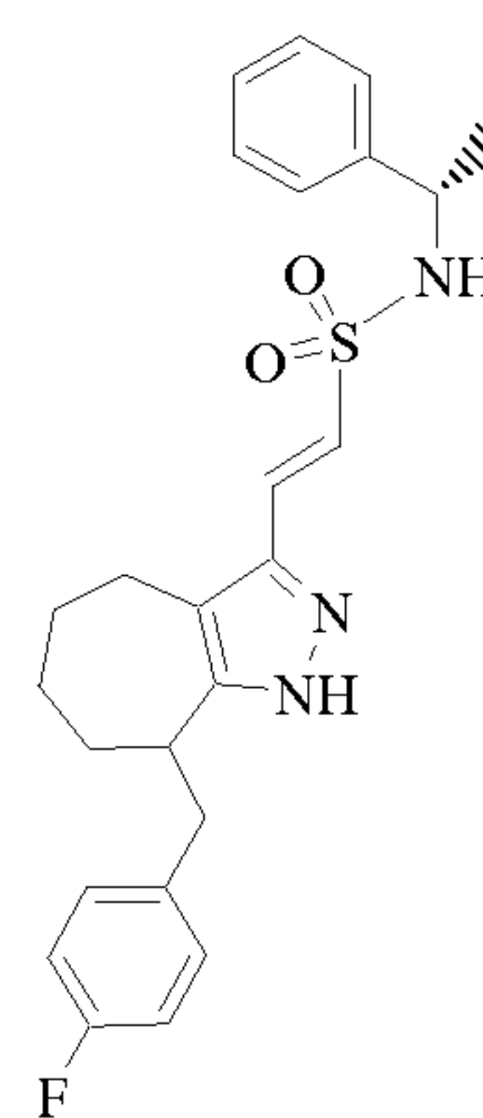
Cpd 104
