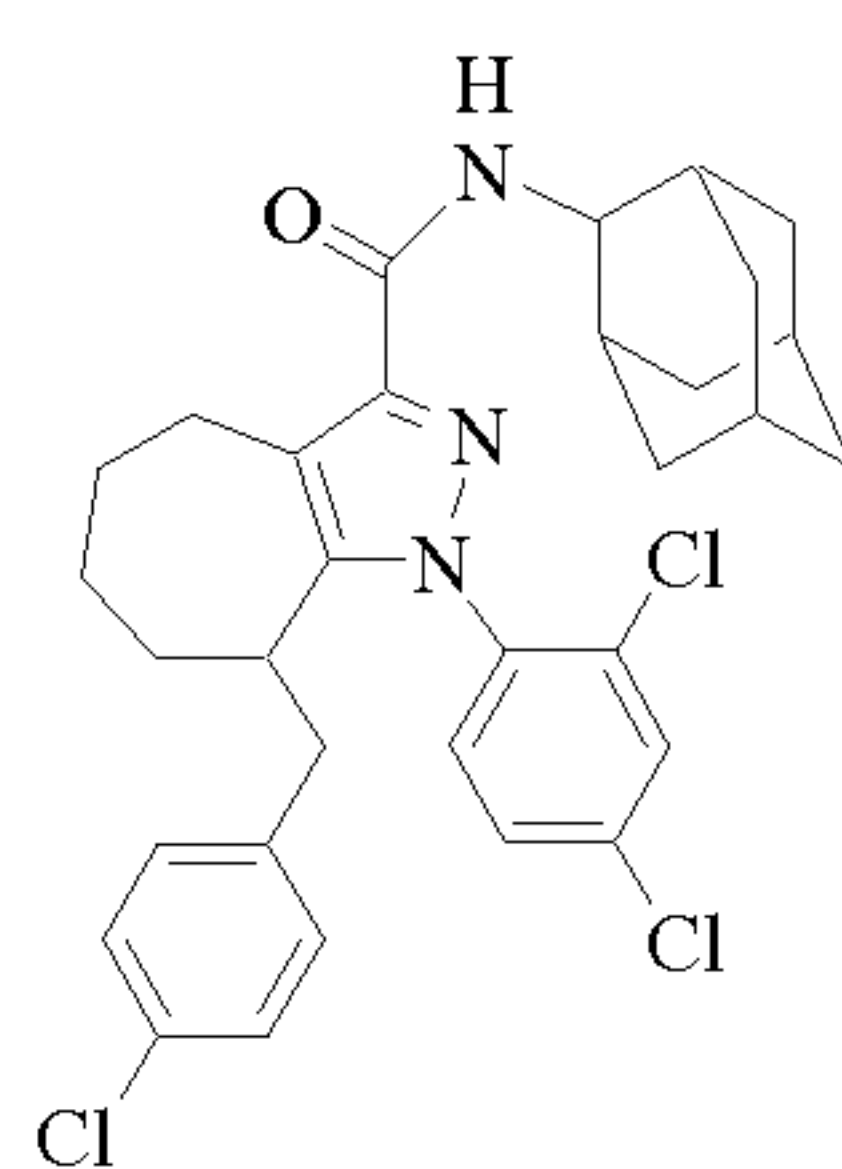
Cpd 14
