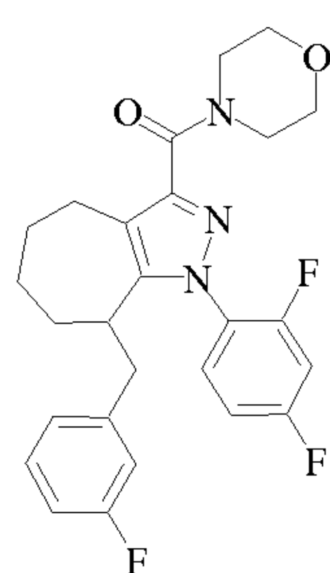
Cpd 114
