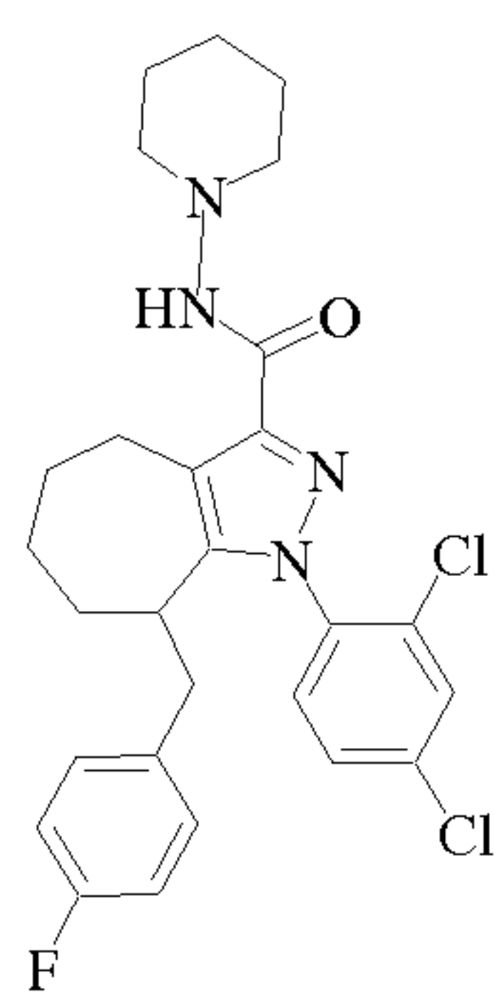
Cpd 85
