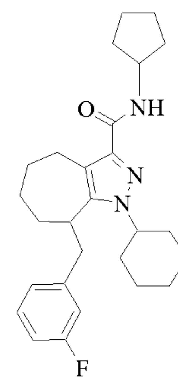
Cpd 52
