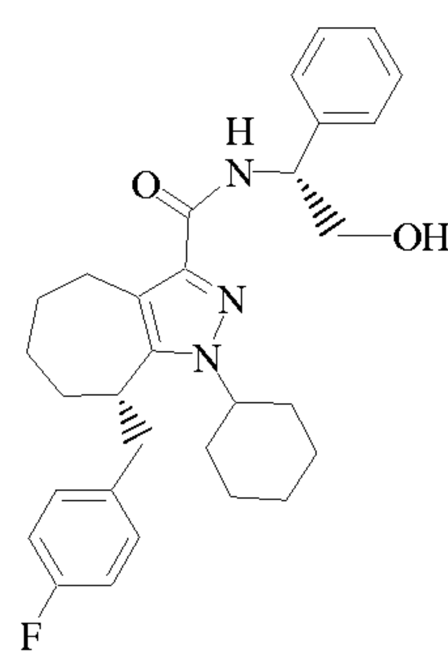
Cpd 63
