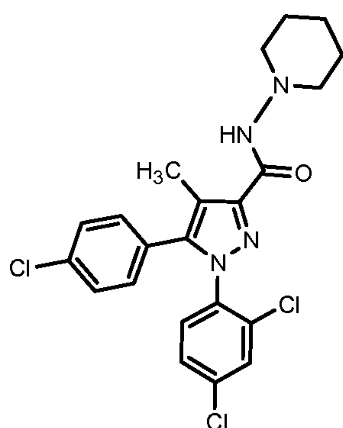
SR 141716
