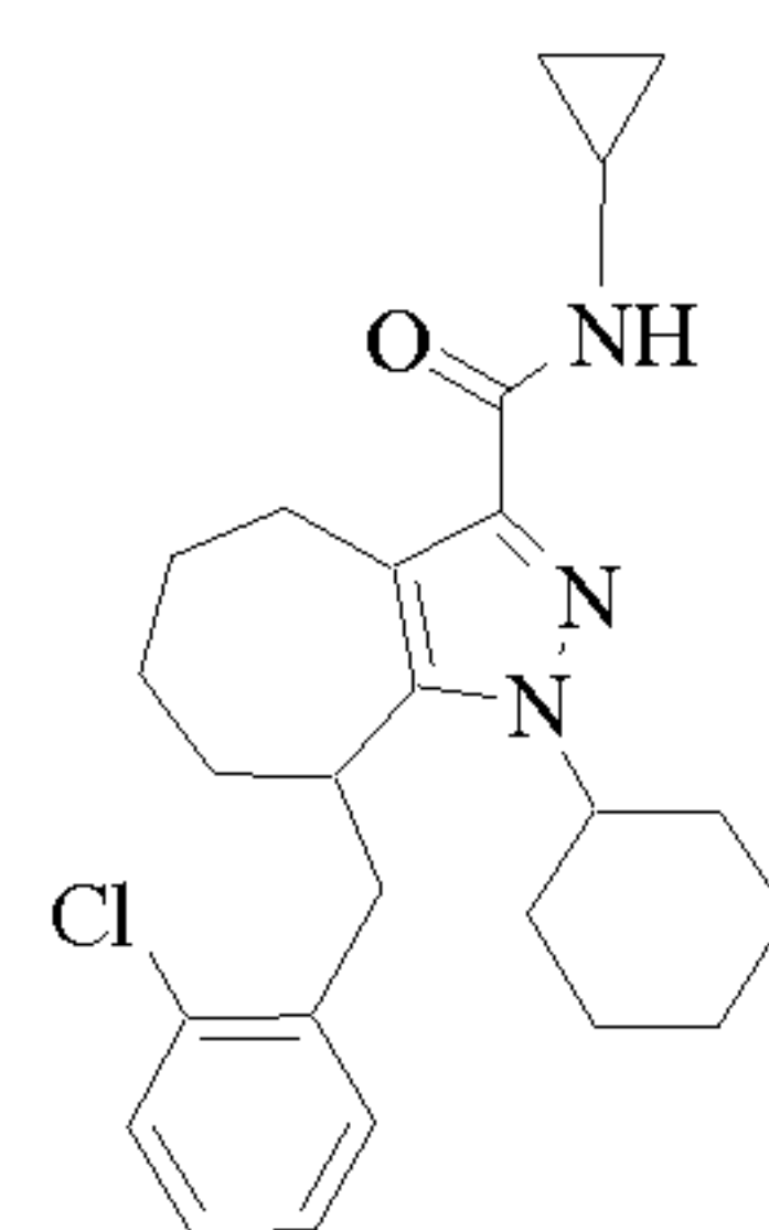
Cpd 31
