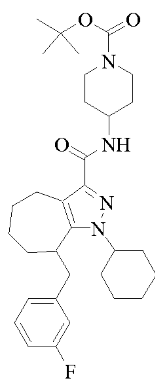
Cpd 46
