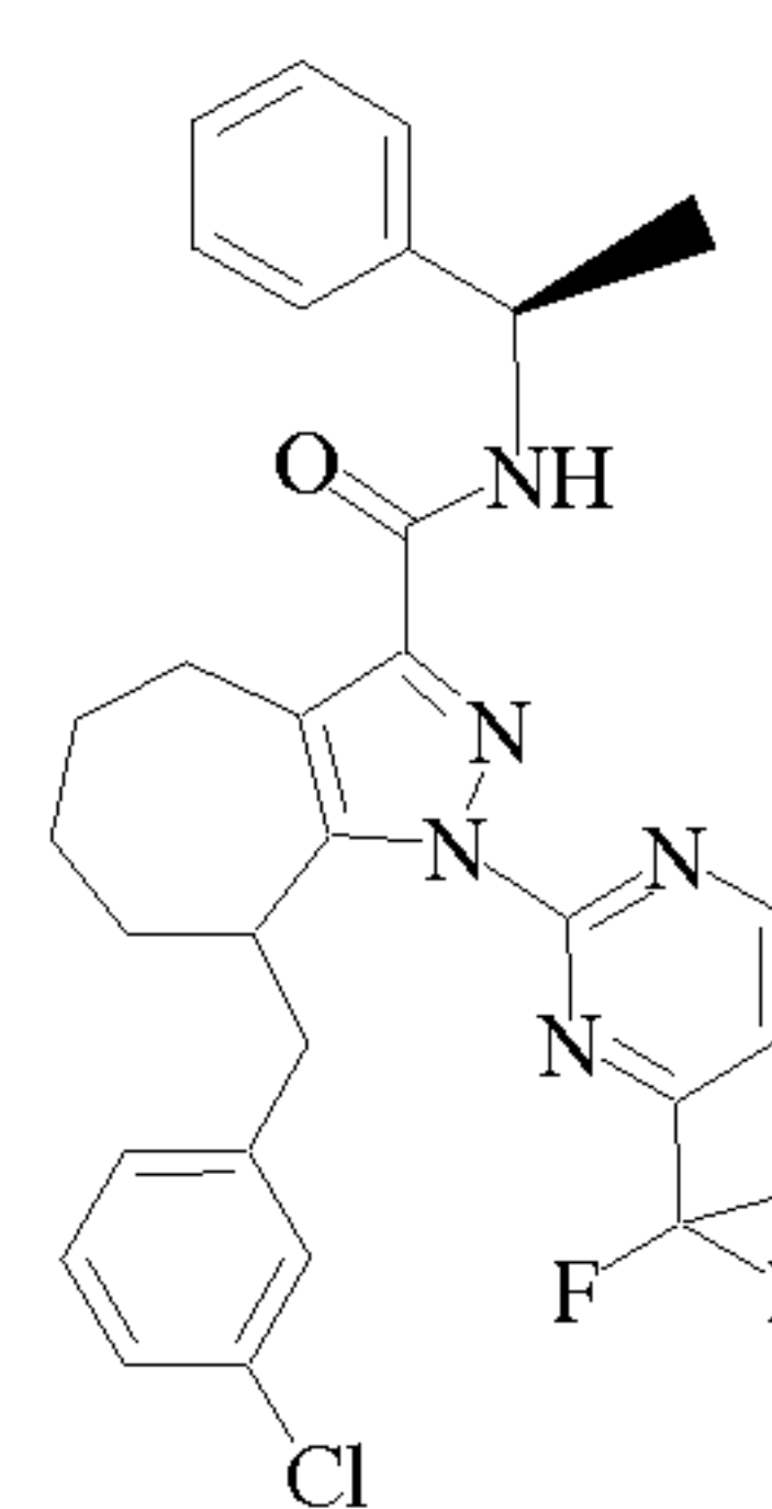
Cpd 175
