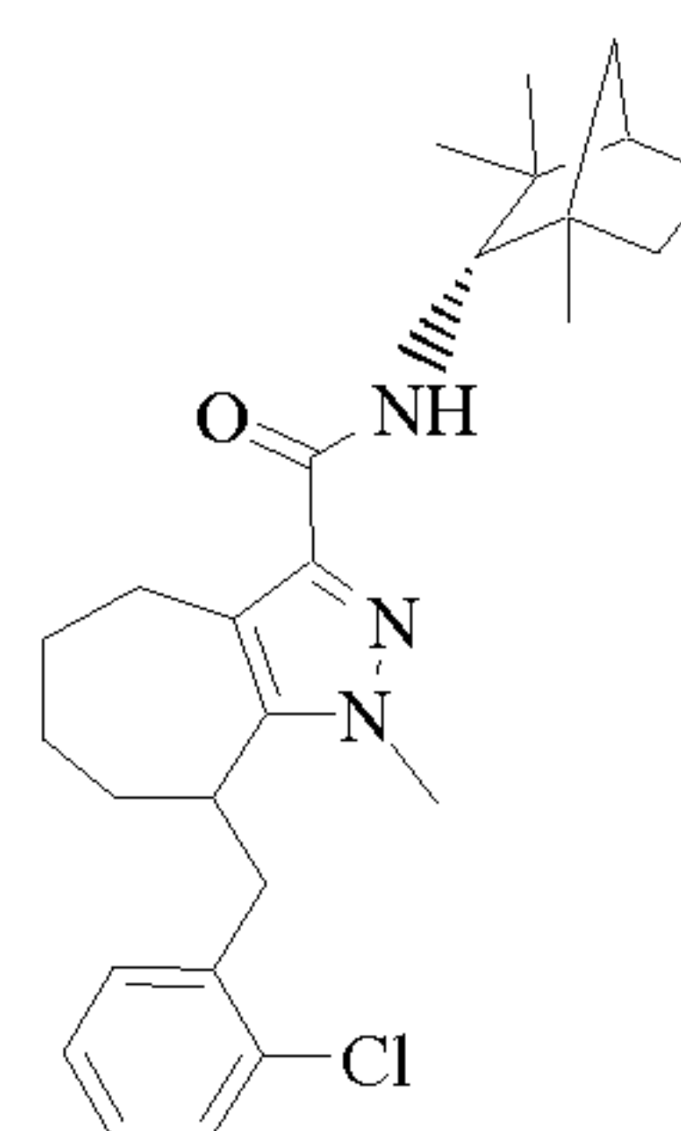
Cpd 40
