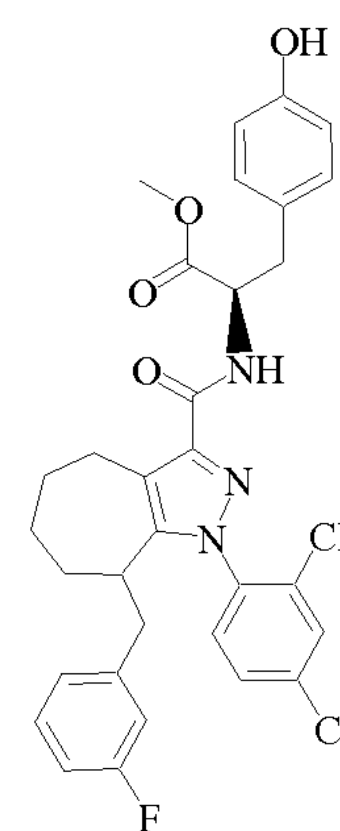
Cpd 80
