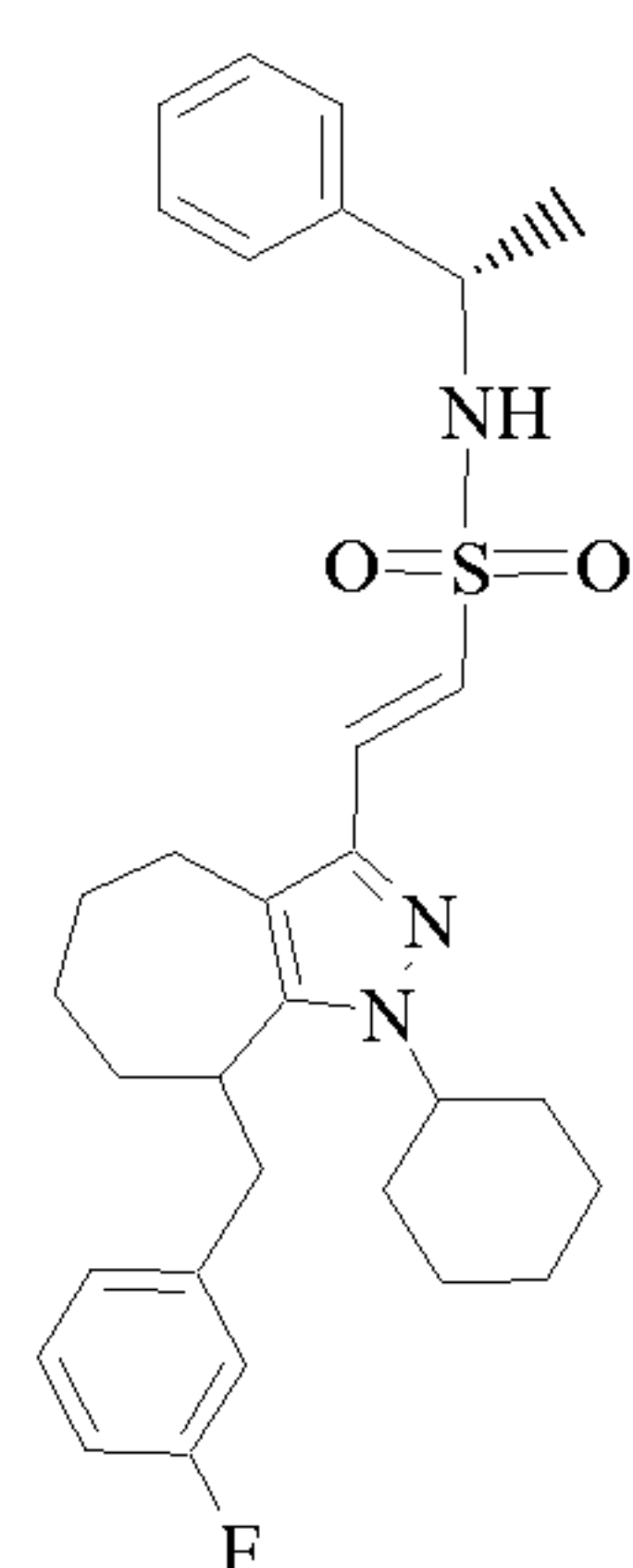
Cpd 75
