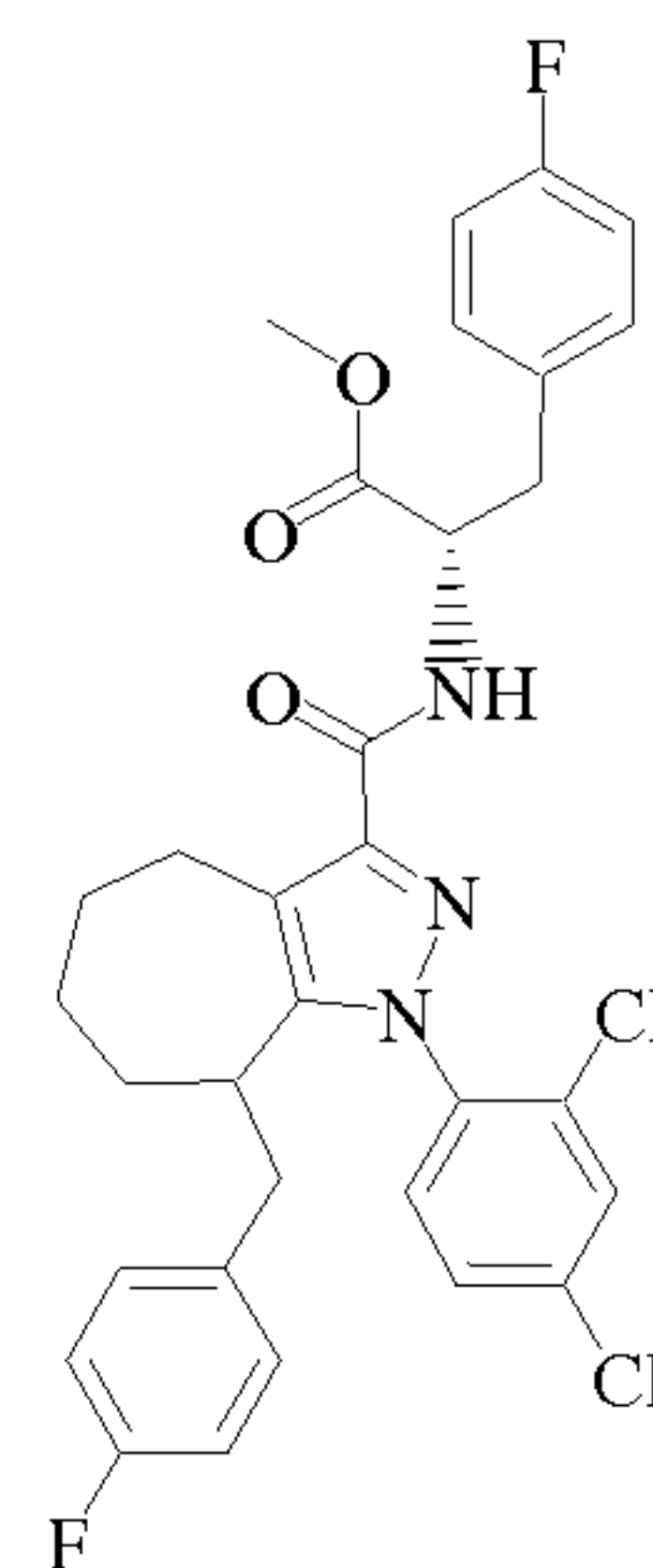
Cpd 72
