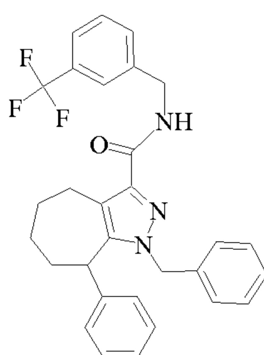
Cpd 65
