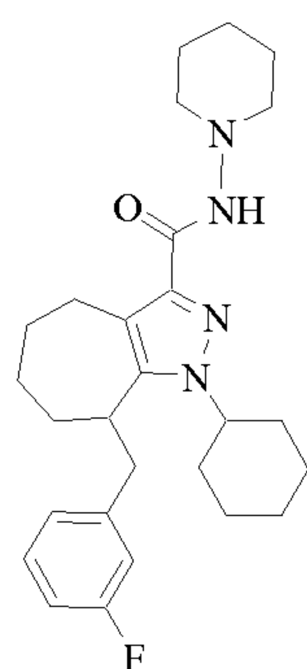
Cpd 50
