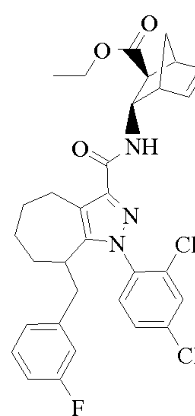
Cpd 75
