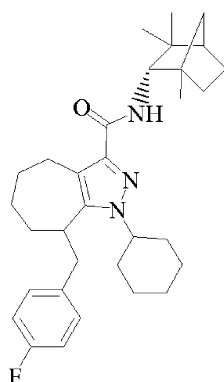
Cpd 58
