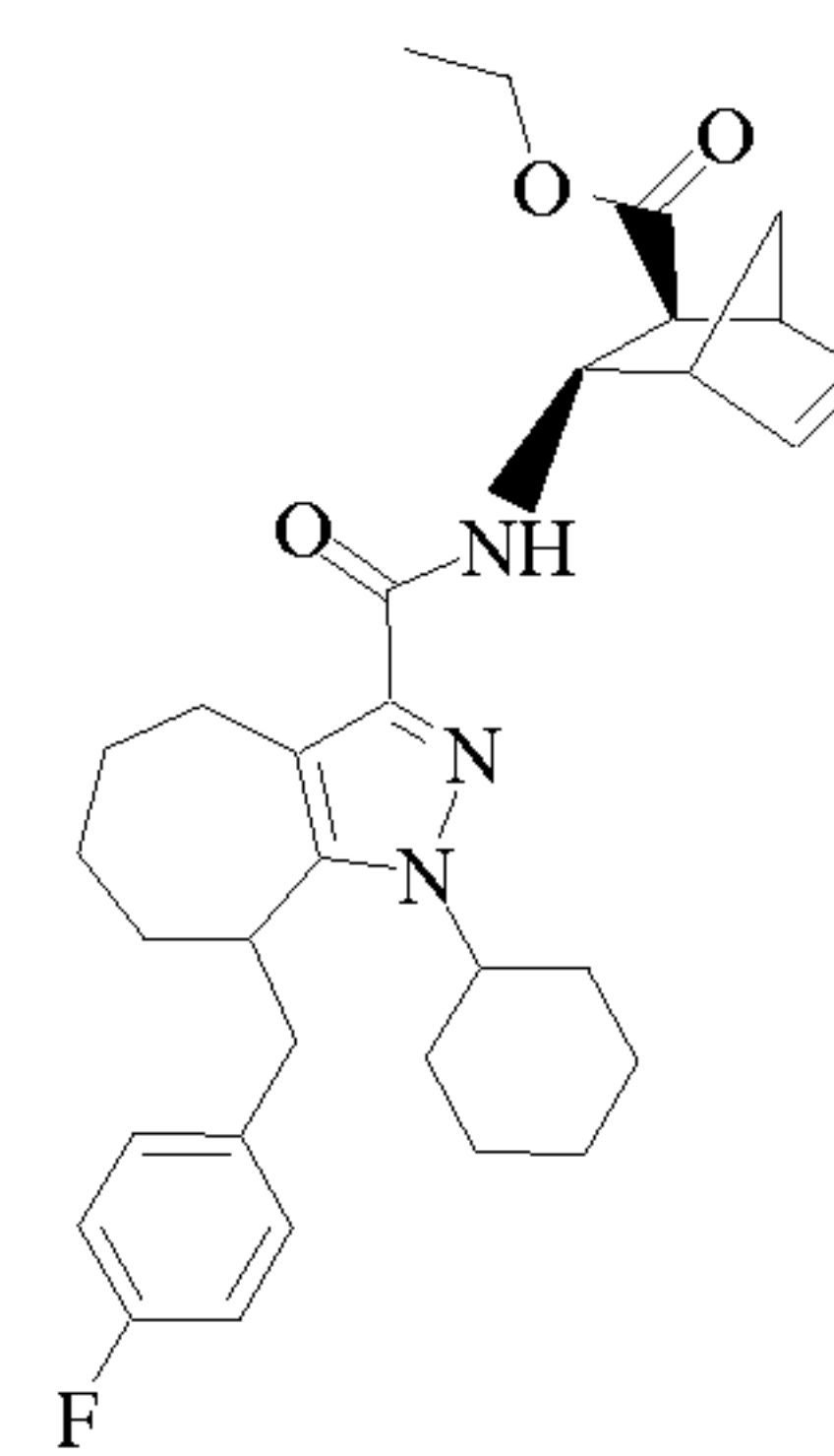
Cpd 88
