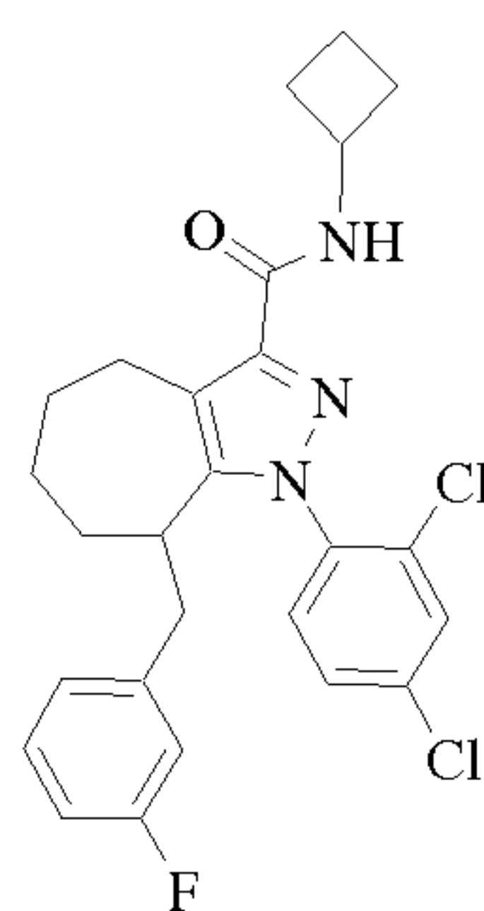
Cpd 37
