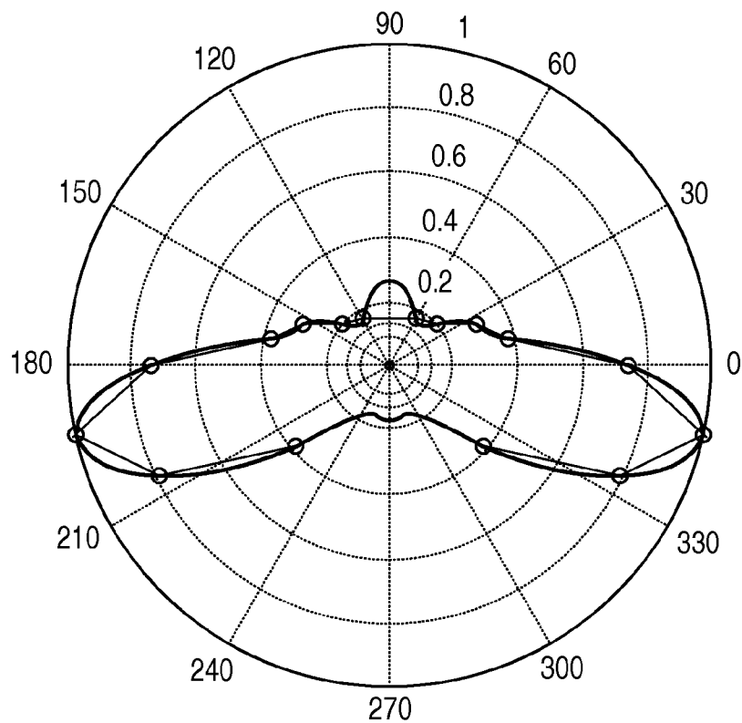
Example of angular domain channel response for a 4-antenna ULA ( M=4 , N=1 )
