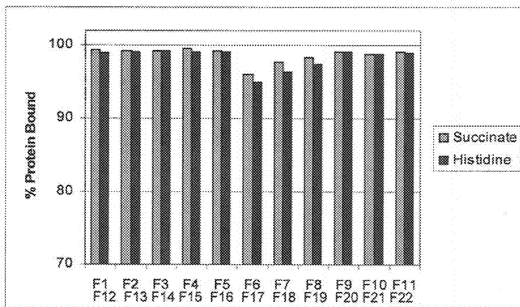
Fig. 26 Binding of Subfamily B with \text{AlPO}_4 in Succinate and Histidine Buffers
