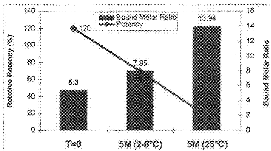
Fig. 17 Correlation of Potency and Bound Molar Ratio for Subfamily B
