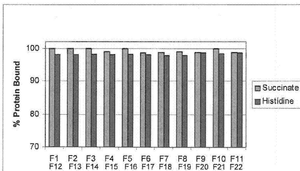
Fig. 25 Binding of Subfamily A with \text{AlPO}_4 in Succinate and Histidine Buffers
