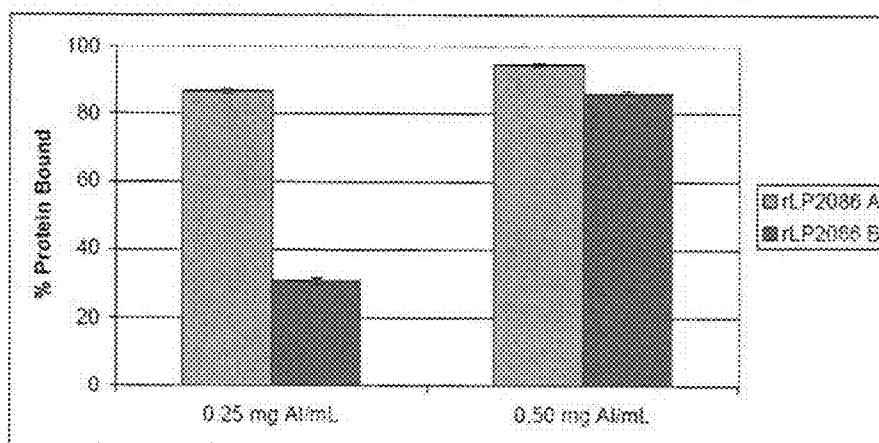
Fig. 7 Protein Binding to Aluminum Phosphate at pH 6.5
