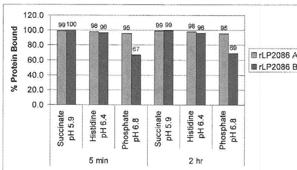
Fig. 27 Comparison of Binding in Succinate, Histidine, and Phosphate buffer
