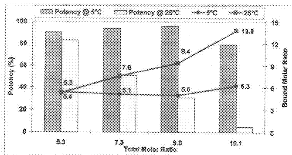
Potency and Bound Molar Ratio Results for Subfamily B
