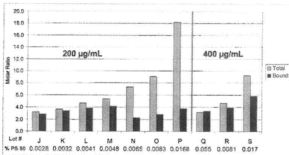
Fig. 19 Molar Ratio Results for Subfamily B
