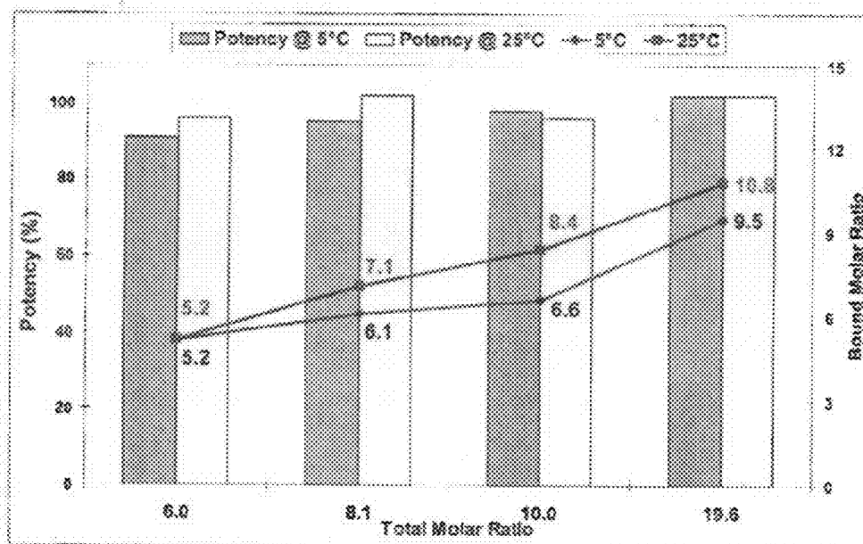
Potency and Bound Molar Ratio Results for Subfamily A
