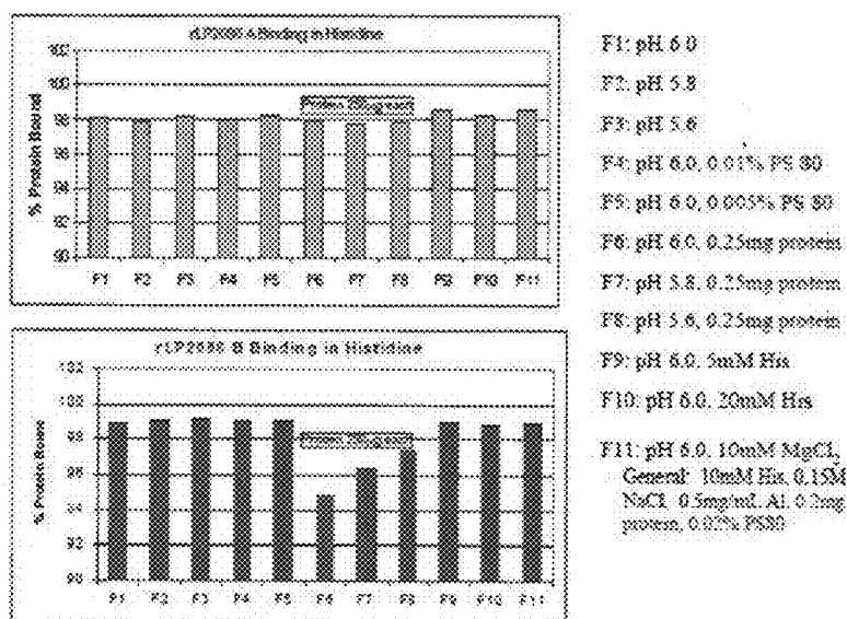
Fig. 9 The Effect of pH, Buffer and Protein Concentration on Binding of rLP2886 Subfamily A and B
