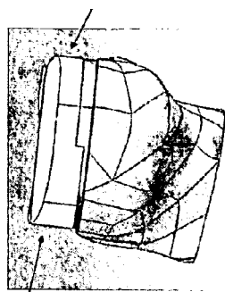
Tibial Cut with AP Sloped of 7° J-Curve is tilted 7° posteriorly to achieve a thicker poly anteriorly
