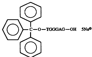
A Compound of Formula 88(a)
