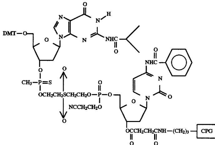
85(a) A Compound of Formula 85(a)
