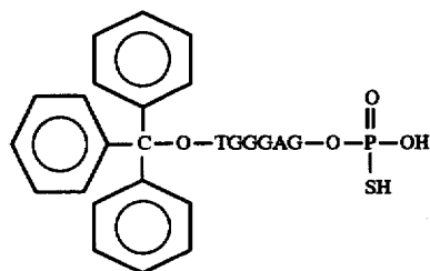
A Compound of Formula 87(a)
