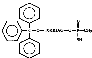
85(b) A Compound of Formula 85(b)
