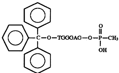
84(b) A. Compound of Formula 84(b)
