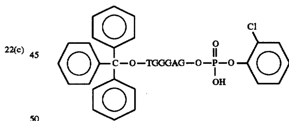
A Compound of Formula 23(a)
