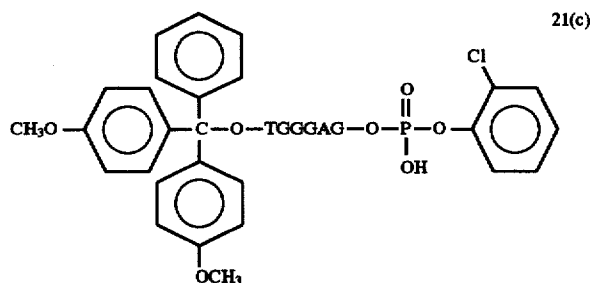
21(c) A Compound of Formula 21(c)
