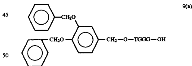
A Compound of Formula 9(a)
