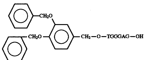
7(c) A Compound of Formula 7(c)
