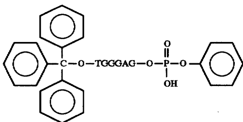
22(c) A Compound of Formula 22(c)
