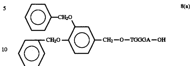
A Compound of Formula 8(a)
