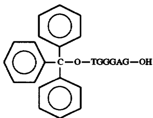
1(b) A Compound of Formula 1(b):
