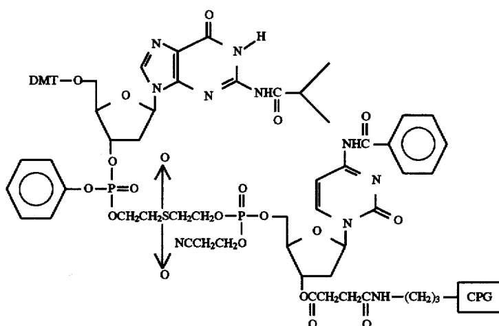
2(b) A Compound of Formula 22(b)
