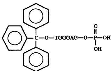
A Compound of Formula 86(a)
