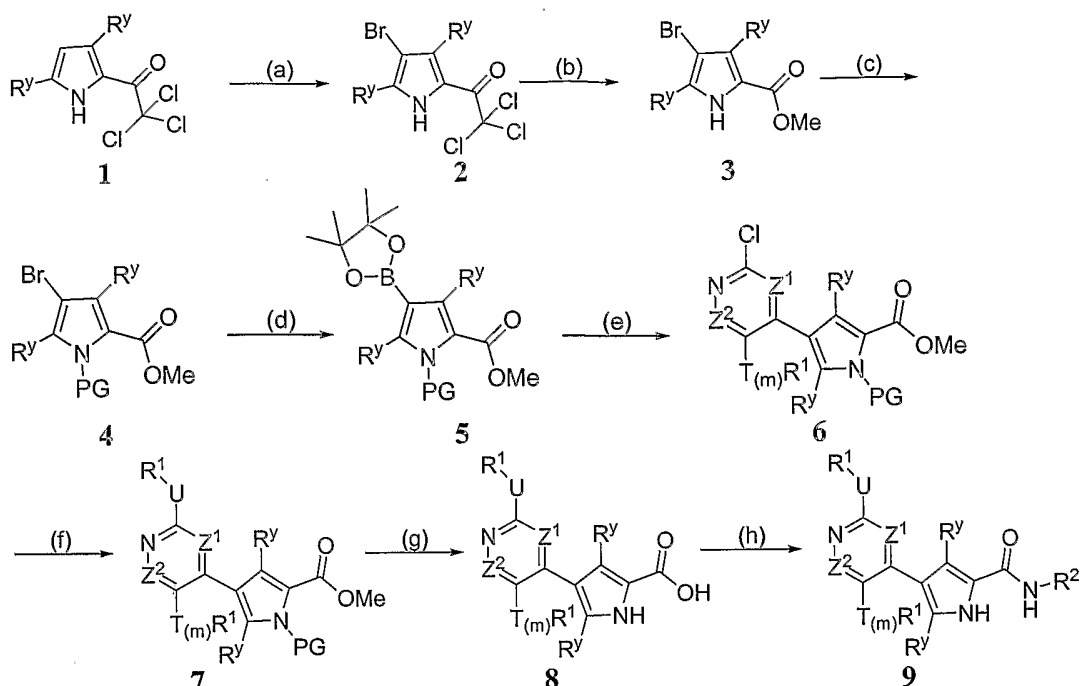
Scheme I
