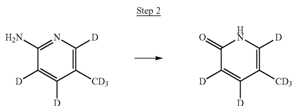
d 6 -5-Methyl-1H-pyridin-2-one
