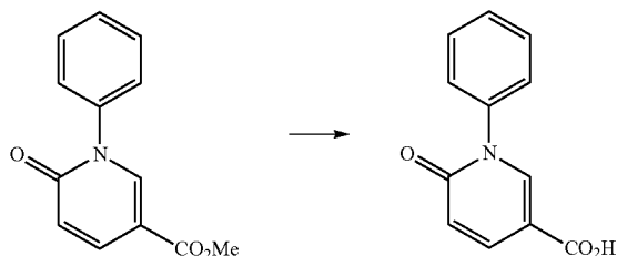
6-Oxo-1-phenyl-1,6-dihydropyridine-3-carboxylic acid
