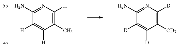
d 6 -5-methylpyridin-2-ylamine
