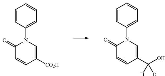
d 2 -5-(Hydroxymethyl)-1-phenylpyridine-2(1H)-one
