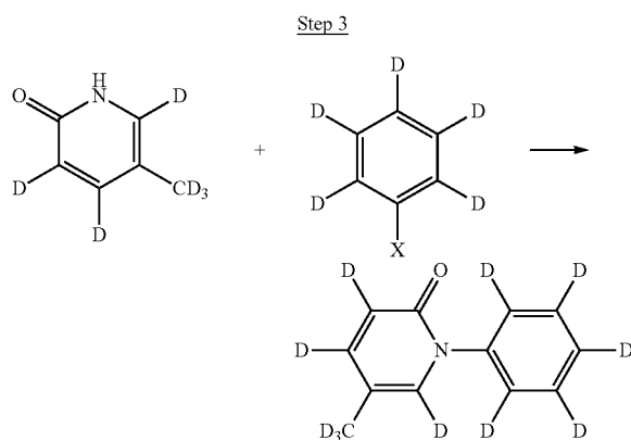
d 11 -5-Methyl-1-phenyl-1H-pyridin-2-one
