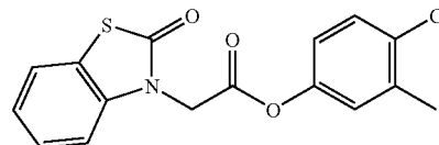
Compound CAS 154184-27-7:
