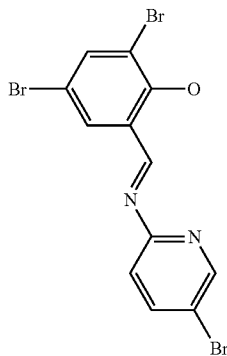
Compound CAS 77367-94-3:
