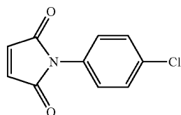
Compound CAS 503065-65-4:
