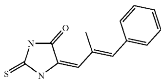
Compound CAS 414908-08:
