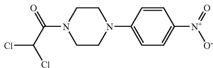
Compound CAS 77367-94-3:
