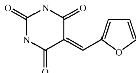
Compound CAS 1631-29-4:
