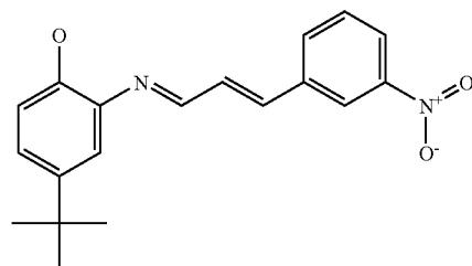
Compound CAS 415703-60-5:
