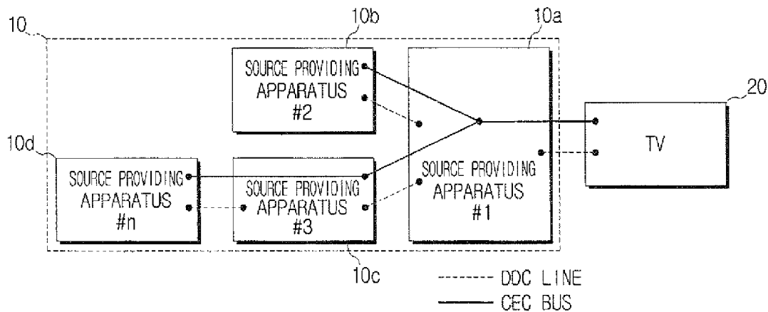
FIG. 2 (RELATED ART)
