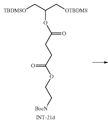
Scheme 21b.
