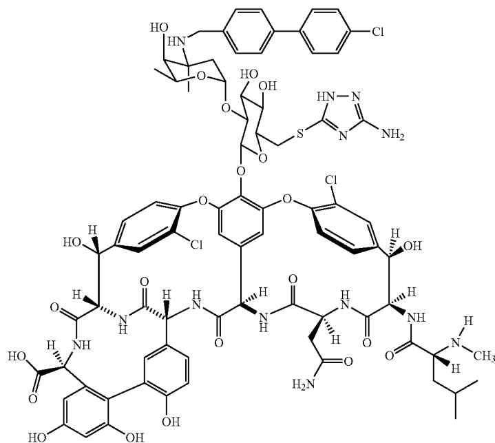
a) Vancosamine-N-4-(4-chlorophenyl)benzyl Glucose-C6-Iodo-Vancomycin (LXXIIIa)
