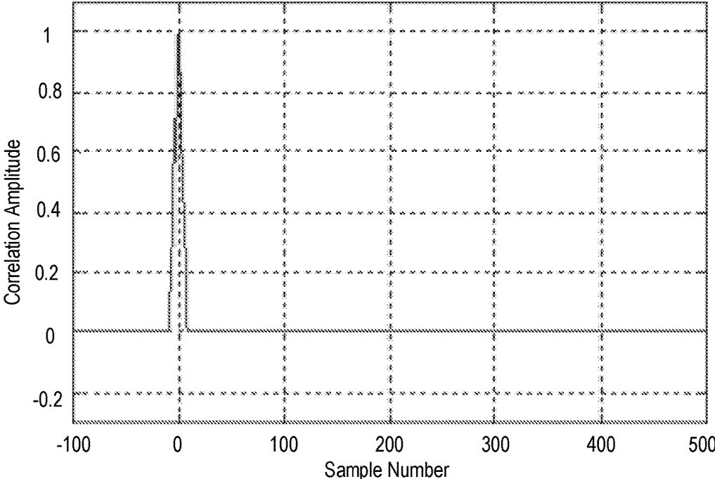
FIG. 4A (Correlation Amplitude, No Notch)
