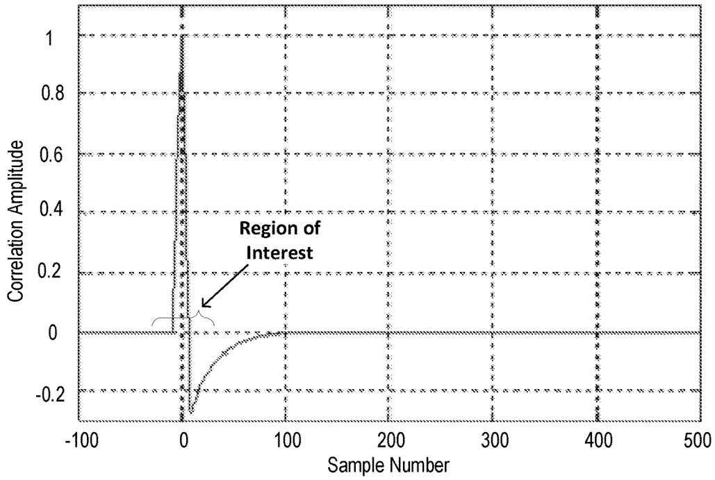
FIG. 4B (Correlation Amplitude, With Notch)
