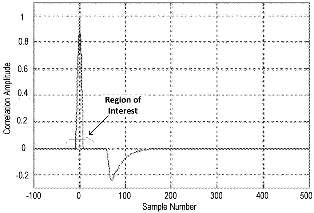
FIG. 4C (Correlation Amplitude, With Modified Notch)
