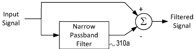
FIG. 3A (Notch Filter)
