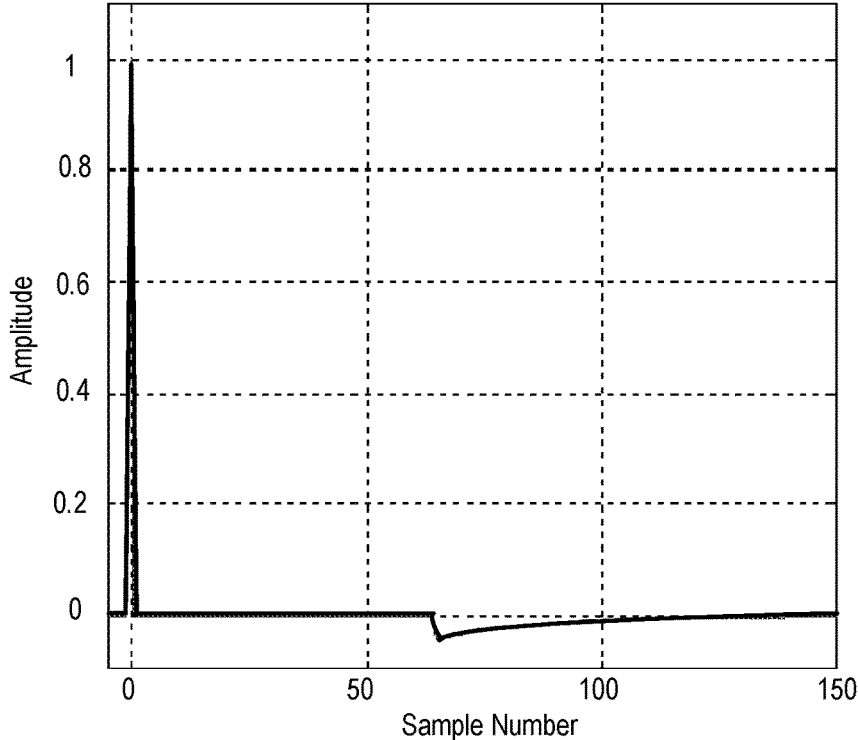
FIG. 2B (Modified Notch Filter Impulse Response)
