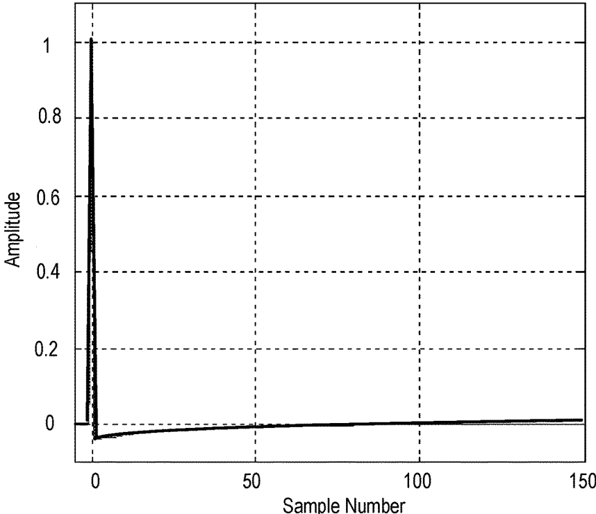
FIG. 2A (Notch Filter Impulse Response)
