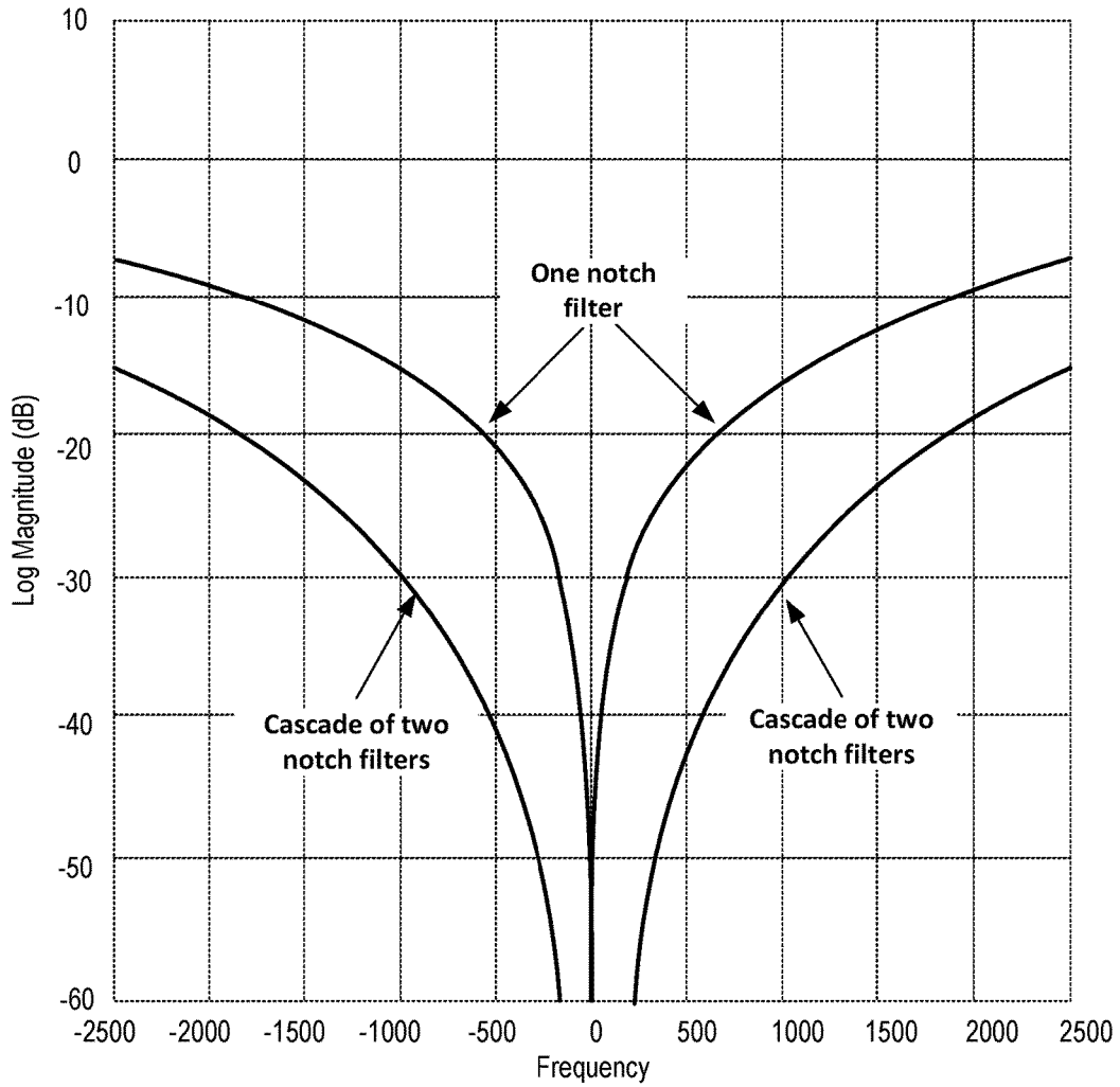
FIG. 6 (Response for One and Two Cascaded Notches)
