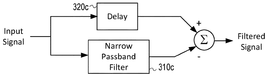
FIG. 3C (Modified Notch Filter With Advanced Passband Filter)
