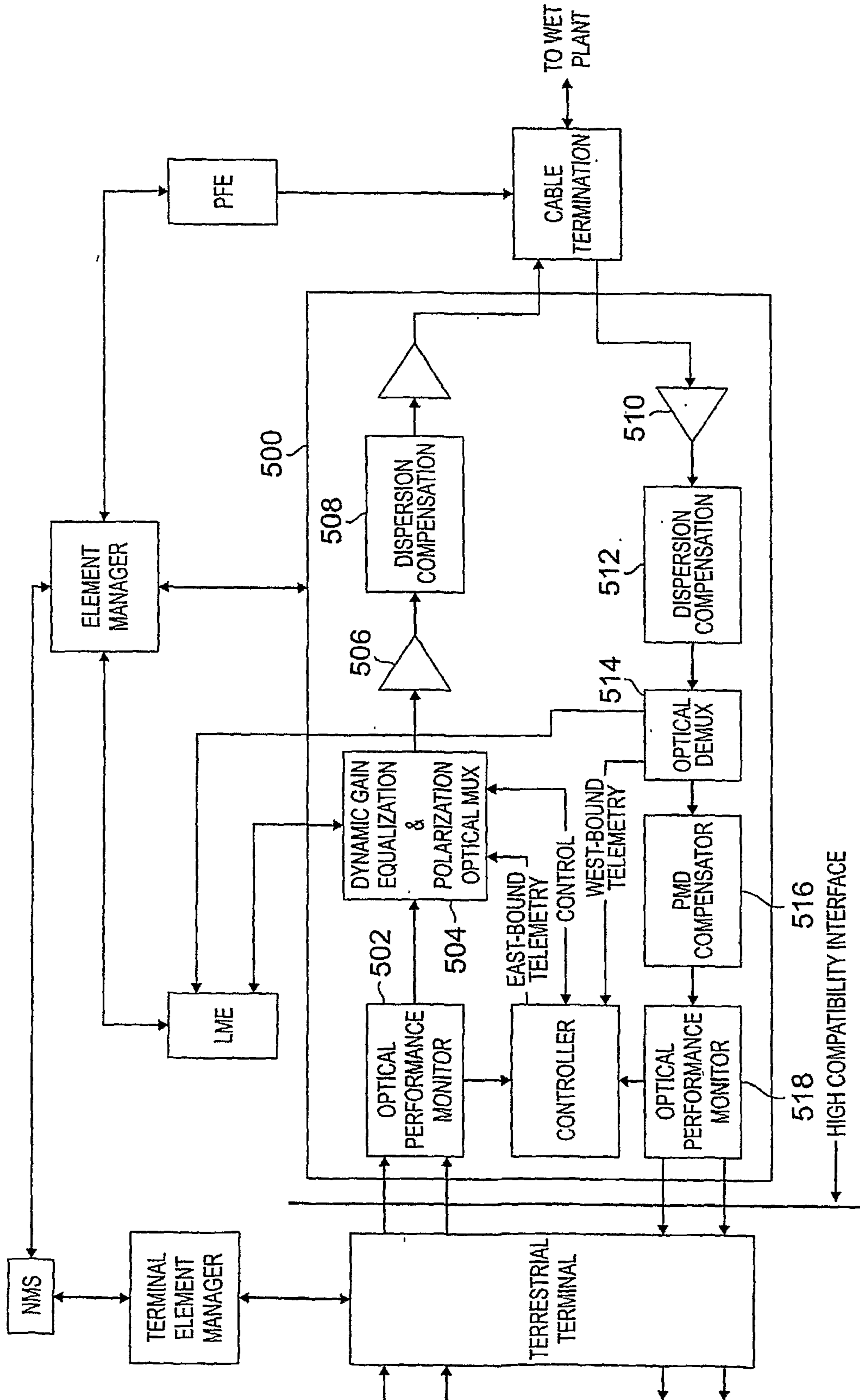
BOLT-ON OPTICAL SIGNAL CONDITIONER BLOCK DIAGRAM
