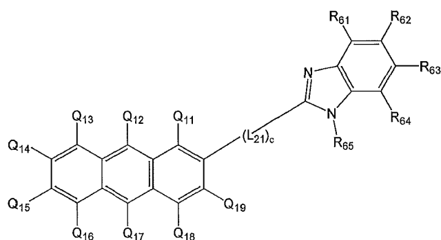
Formula 4
