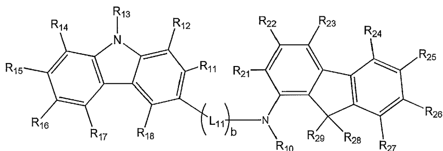
Formula 2
