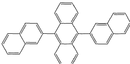
Compound 60
