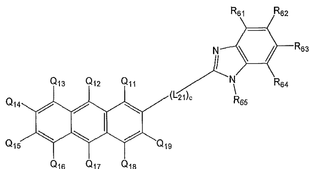
Formula 4
