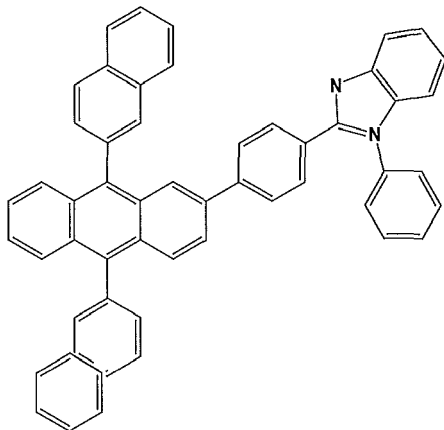
Compound 61
