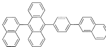
Compound 52
