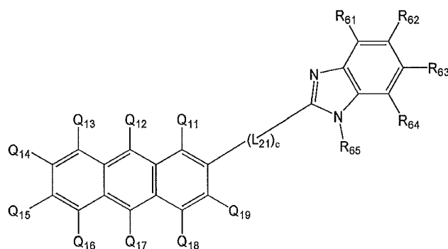
Formula 4
