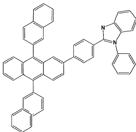
Compound 61
