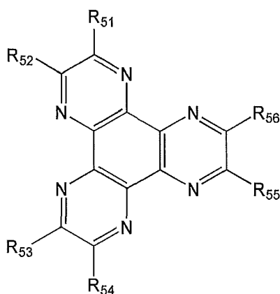
Formula 3
