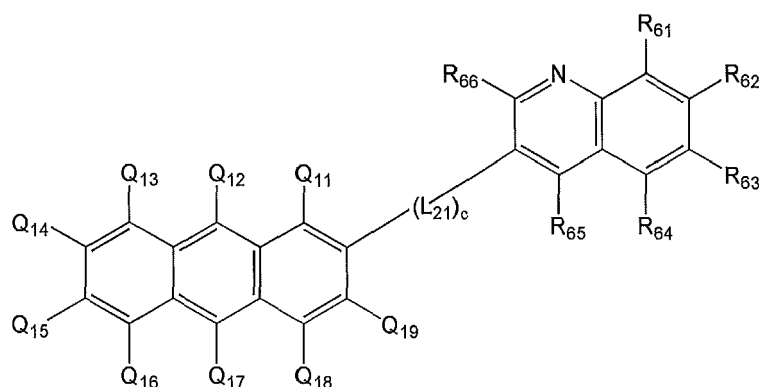
Formula 5
