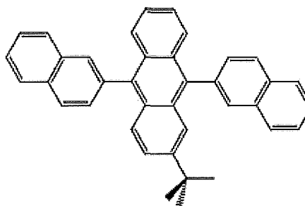
TBADN
