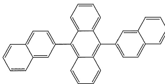
ADN
