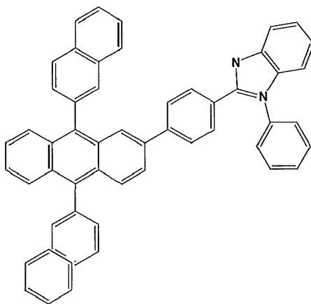
Compound 61
