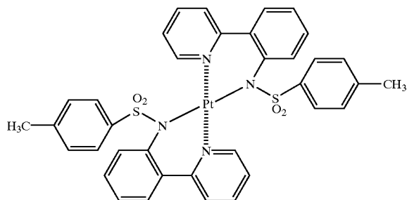
(Compound 17)
