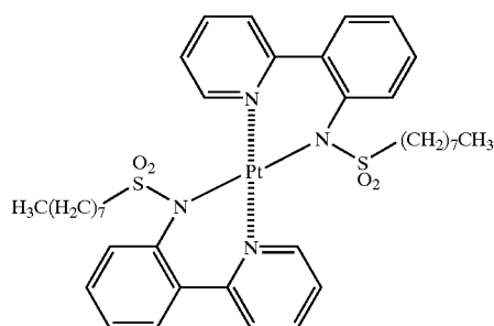
(Compound 18)
