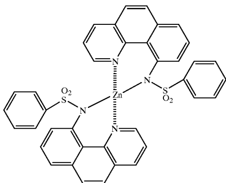
(Compound 14)
