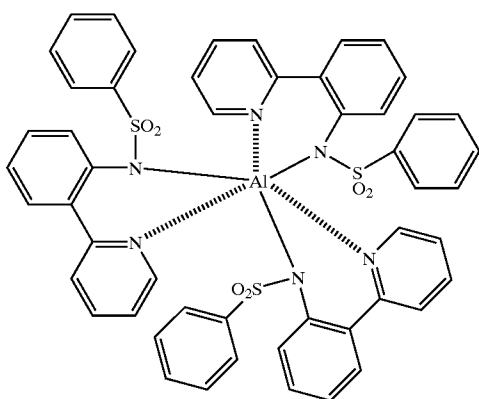
(Compound 16)
