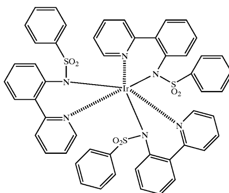
(Compound 19)
