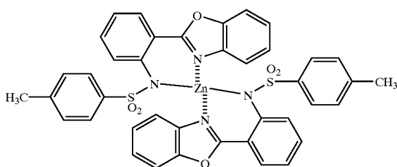
(Compound 2a)
