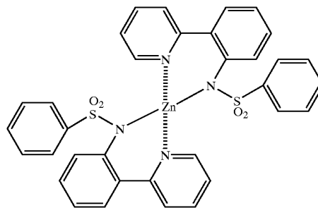
(Compound 2)
