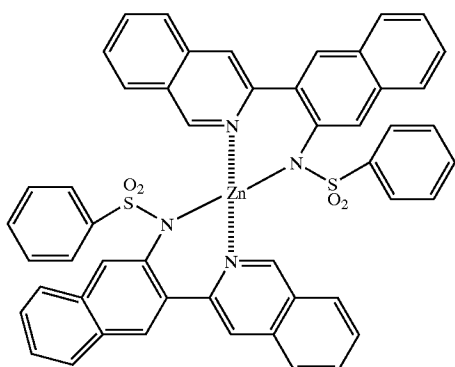
(Compound 15)
