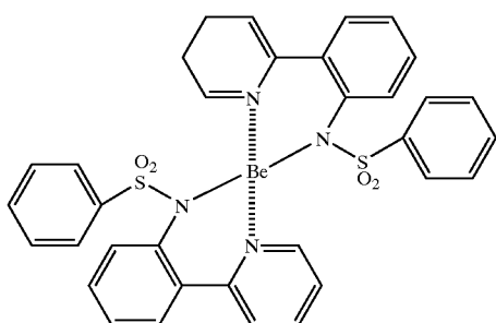
(Compound 16)
