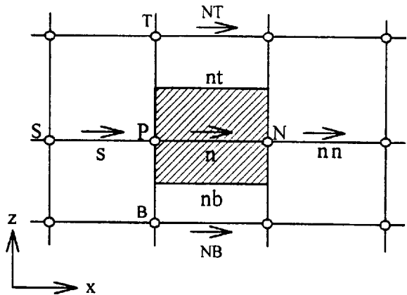
(b) X2 (z) staggered grid
