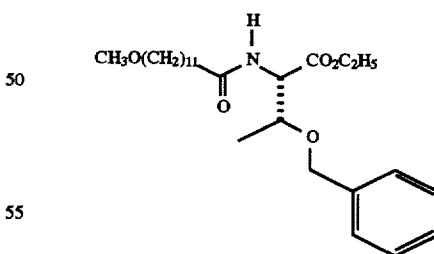
N-(12-methoxy-1-oxododecyl)-O-(phenylmethyl)-L-threonine, Ethyl ester
