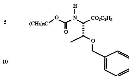
N-(t-Butyloxycarbonyl)-O-(phenylmethyl)-L-threonine, Ethyl ester
