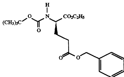
N-(t-Butyloxycarbonyl)-D-glutamic acid, 1-Ethyl 5-(Phenylmethyl)ester
