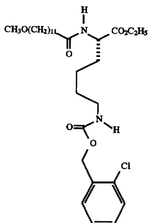
N6-[[2-Chlorophenyl)methoxy]carbonyl]-N2-(12-methoxy-1-oxododecyl)-L-lysine, Ethyl ester
