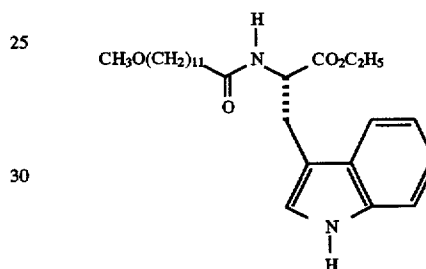
N-(12-Methoxy-1-oxododecyl)-L-tryptophan, Ethyl ester
