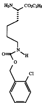
N6-[[2-Chlorophenyl)methoxy]carbonyl]-L-lysine, Ethyl ester Trifluoroacetate
