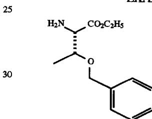
O-(Phenylmethyl)-L-threonine, Ethyl ester Trifluoroacetate
