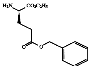
D-glutamic acid, 1-Ethyl 5-(Phenylmethyl)ester Trifluoroacetate
