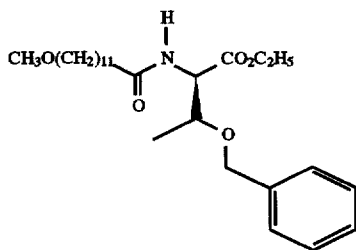
N-(12-methoxy-1-oxododecyl)-O-(phenylmethyl)-D-threonine, Ethyl ester
