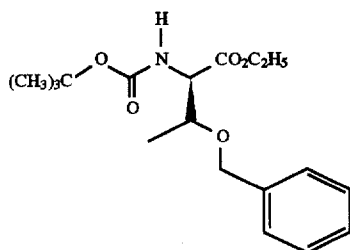
N-(t-Butyloxycarbonyl)-O-(phenylmethyl)-D-threonine, Ethyl ester
