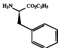
D-Phenylalanine Ethyl ester p-Toluenesulfonate
