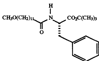
N-(12-Methoxy-1-oxododecyl)-L-phenylalanine, 1, 1-Dimethylethyl ester
