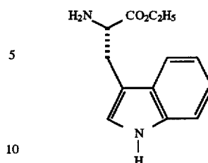
L-Tryptophan Ethyl ester Trifluoroacetate
