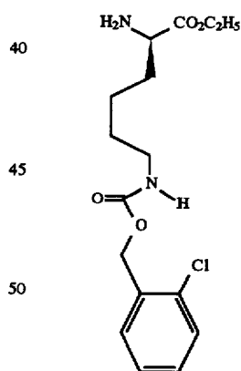
N6-[[2-Chlorophenyl)methoxy]carbonyl]-N2-(12-methoxy-1-oxododecyl)-L-lysine, Ethyl ester
