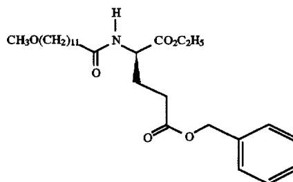
N-(12-methoxy-1-oxododecyl)-D-glutamic acid, 1-Ethyl 5-(Phenylmethyl)ester
