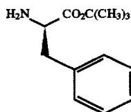
D-Phenylalanine 1,1-Dimethylethyl ester
