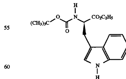
N-(t-Butyloxycarbonyl)-D-tryptophan, Ethyl ester
