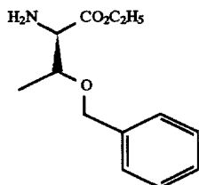
O-(Phenylmethyl)-D-threonine, Ethyl ester Trifluoroacetate
