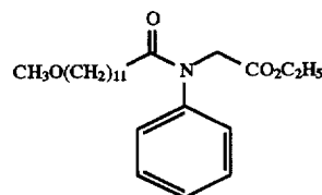
N-(12-Methoxy-1-oxododecyl)-N-phenylglycine, Ethyl ester
