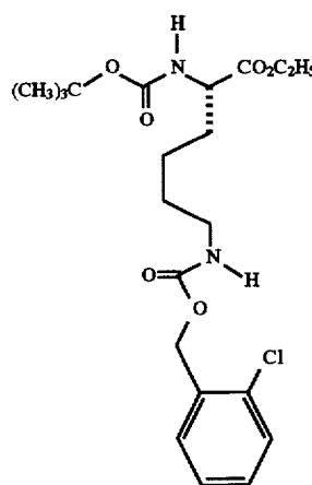
N6-[[[(2-Chlorophenyl)methoxy]carbonyl]-N2-[t-butylloxycarbonyl]-L-lysine, Ethyl ester
