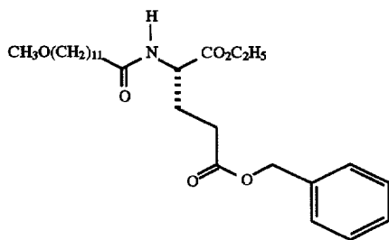
N-(12-methoxy-1-oxododecyl)-L-glutamic acid, 1-Ethyl 5-(Phenylmethyl)ester
