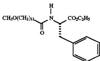
N-(12-Methoxy-1-oxododecyl)-L-phenylalanine, Ethyl ester
