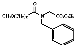
N-(12-Methoxy-1-oxododecyl)-N-(phenylmethyl)-glycine, Ethyl ester
