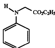
N-phenylglycine, Ethyl ester
