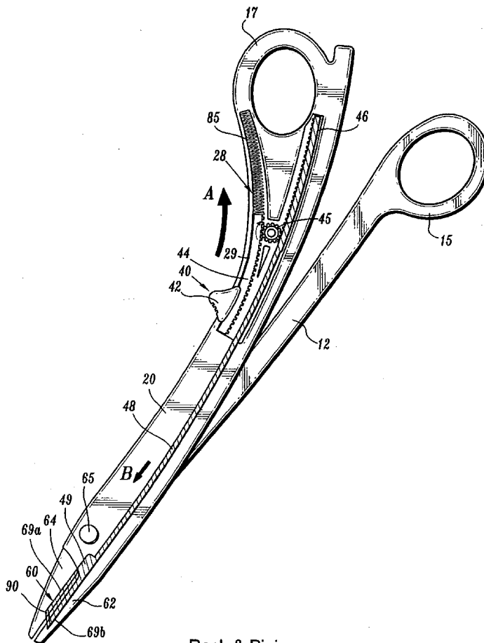
Rack & Pinion
