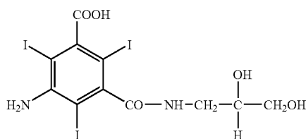
5-amino-2,4,6-triodophthalic acid-(2,3-dihydroxypropyl)-amide (ATH)
