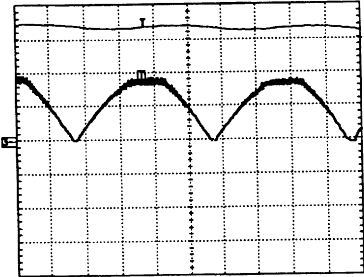
Actual Output Voltage and Rectified V_{in} (50V/div) [Timebase=2.5ms/div]
