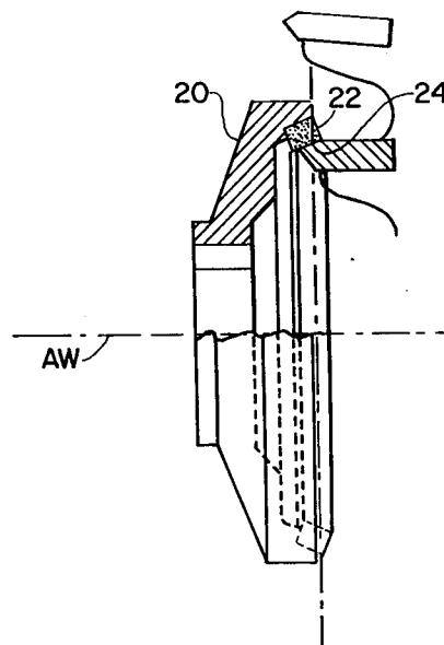
FIG. 4 PRIOR ART
