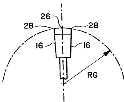
FIG. 3F PRIOR ART
